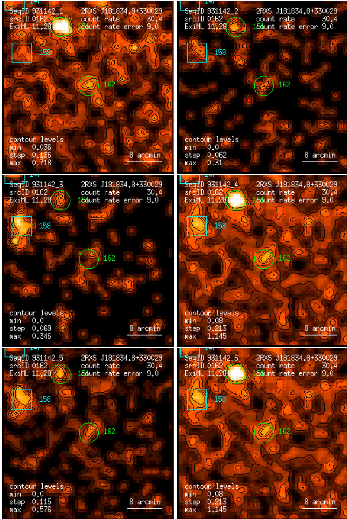
Figure 162: RASS 931142: detection 0162: band rate images, Gaussian filter: (1) PSPC channels 11 – 41, (2) 52 – 90, (3) 91 – 201, (4) 11 – 235, (5) 52 – 201, (6) 11 – 201. Broad band rates in counts/ks. Band rate contour levels in counts/ks/arcmin 2 .
