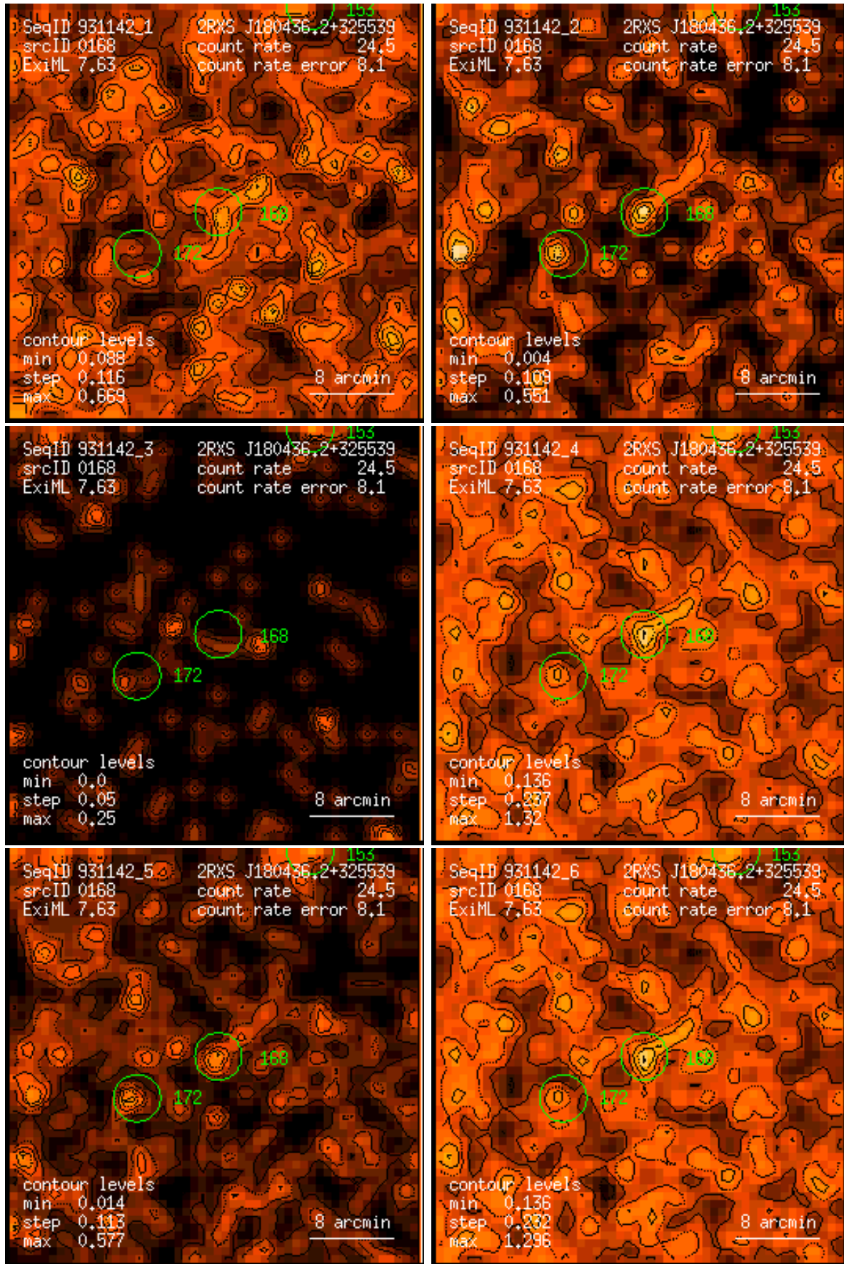
Figure 168: RASS 931142: detection 0168: band rate images, Gaussian filter: (1) PSPC channels 11 – 41, (2) 52 – 90, (3) 91 – 201, (4) 11 – 235, (5) 52 – 201, (6) 11 – 201. Broad band rates in counts/ks. Band rate contour levels in counts/ks/arcmin 2 .
