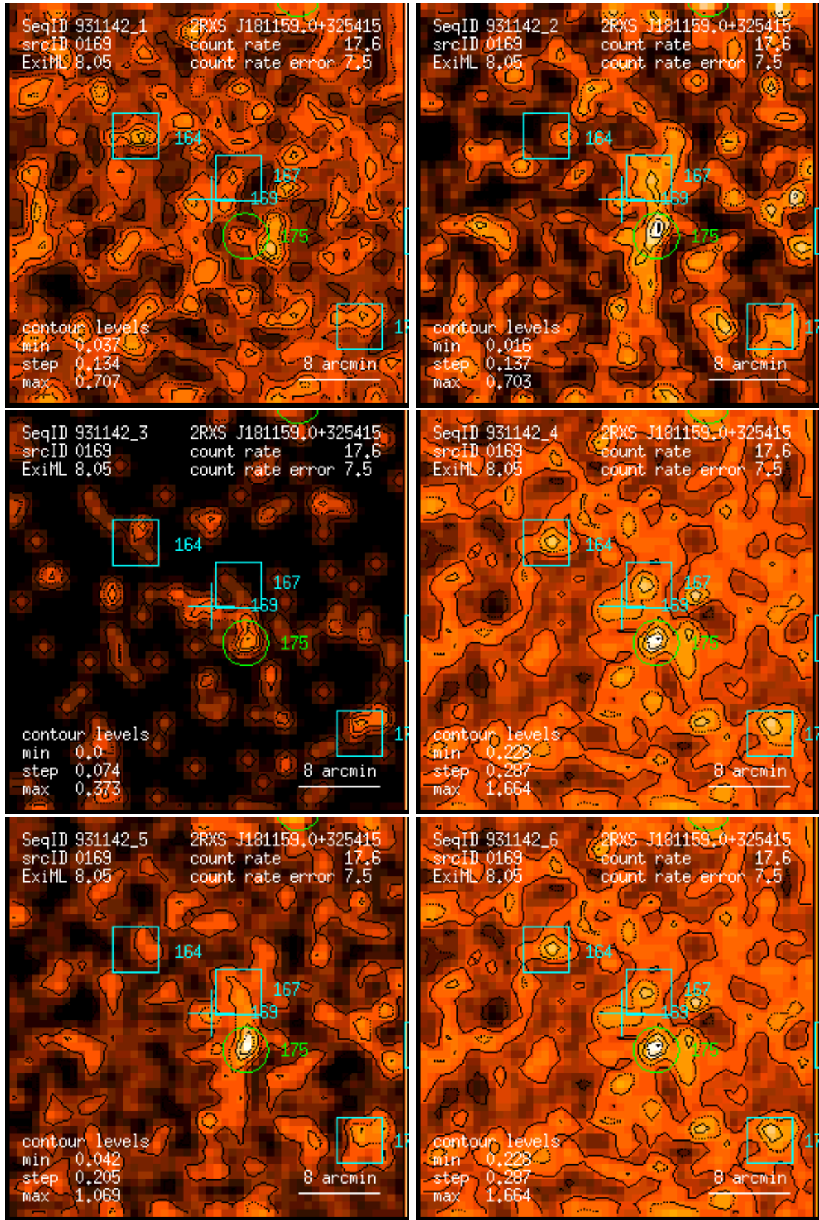
Figure 169: RASS 931142: detection 0169: band rate images, Gaussian filter: (1) PSPC channels 11 – 41, (2) 52 – 90, (3) 91 – 201, (4) 11 – 235, (5) 52 – 201, (6) 11 – 201. Broad band rates in counts/ks. Band rate contour levels in counts/ks/arcmin 2 .
