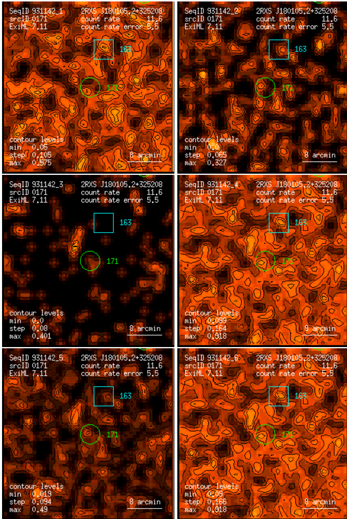
Figure 171: RASS 931142: detection 0171: band rate images, Gaussian filter: (1) PSPPC channels 11 – 41, (2) 52 – 90, (3) 91 – 201, (4) 11 – 235, (5) 52 – 201, (6) 11 – 201. Broad band rates in counts/ks. Band rate contour levels in counts/ks/arcmin 2 .
