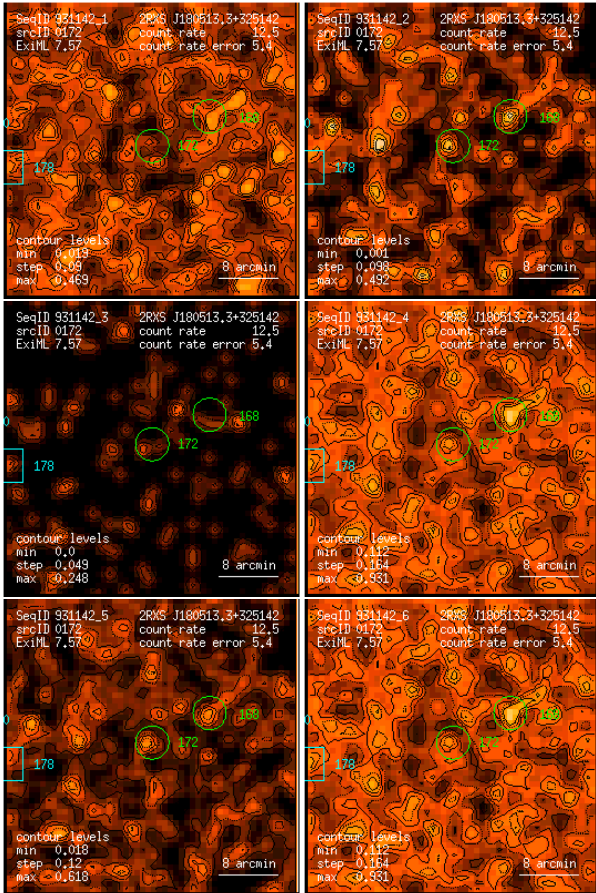
Figure 172: RASS 931142: detection 0172: band rate images, Gaussian filter: (1) PSPC channels 11 – 41, (2) 52 – 90, (3) 91 – 201, (4) 11 – 235, (5) 52 – 201, (6) 11 – 201. Broad band rates in counts/ks. Band rate contour levels in counts/ks/arcmin 2 .
