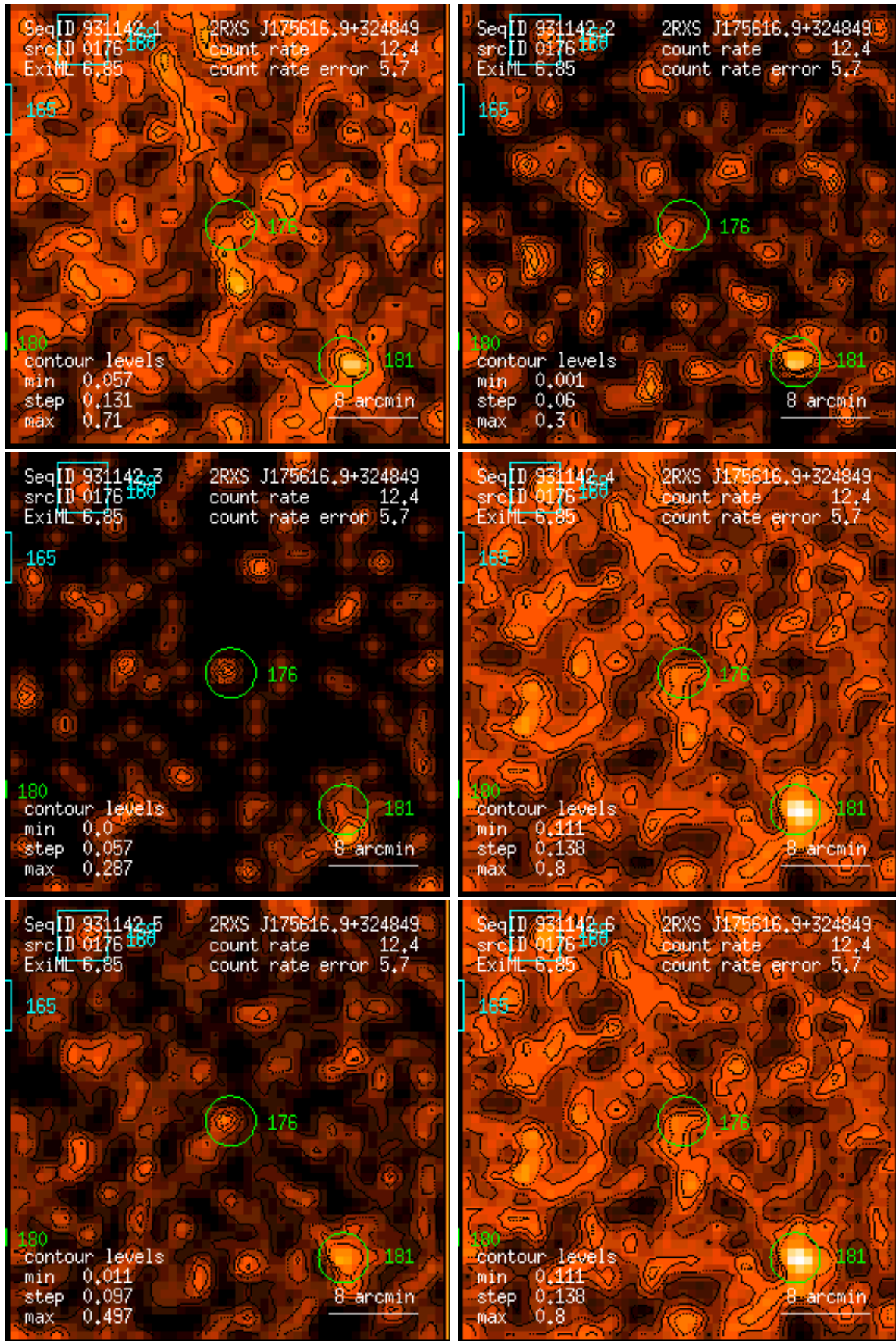
Figure 176: RASS 931142: detection 0176: band rate images, Gaussian filter: (1) PSPC channels 11 – 41, (2) 52 – 90, (3) 91 – 201, (4) 11 – 235, (5) 52 – 201, (6) 11 – 201. Broad band rates in counts/ks. Band rate contour levels in counts/ks/arcmin 2 .
