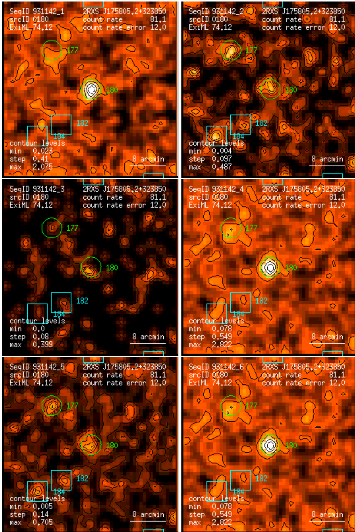
Figure 180: RASS 931142: detection 0180: band rate images, Gaussian filter: (1) PSPC channels 11 – 41, (2) 52 – 90, (3) 91 – 201, (4) 11 – 235, (5) 52 – 201, (6) 11 – 201. Broad band rates in counts/ks. Band rate contour levels in counts/ks/arcmin 2 .
