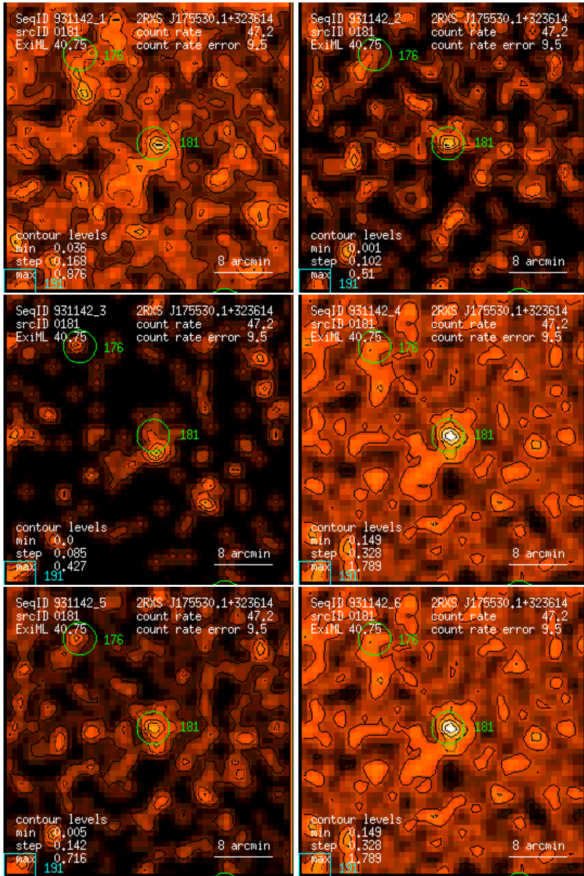
Figure 181: RASS 931142: detection 0181: band rate images, Gaussian filter: (1) PSPC channels 11 – 41, (2) 52 – 90, (3) 91 – 201, (4) 11 – 235, (5) 52 – 201, (6) 11 – 201. Broad band rates in counts/ks. Band rate contour levels in counts/ks/arcmin 2 .
