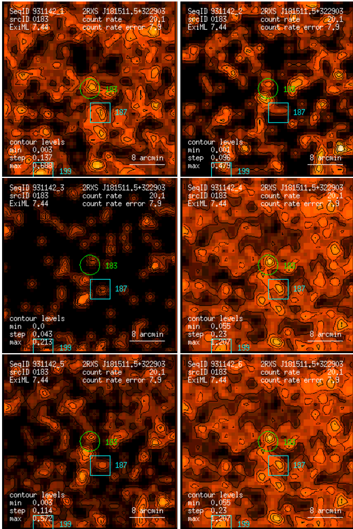
Figure 183: RASS 931142: detection 0183: band rate images, Gaussian filter: (1) PSPC channels 11 – 41, (2) 52 – 90, (3) 91 – 201, (4) 11 – 235, (5) 52 – 201, (6) 11 – 201. Broad band rates in counts/ks. Band rate contour levels in counts/ks/arcmin 2 .
