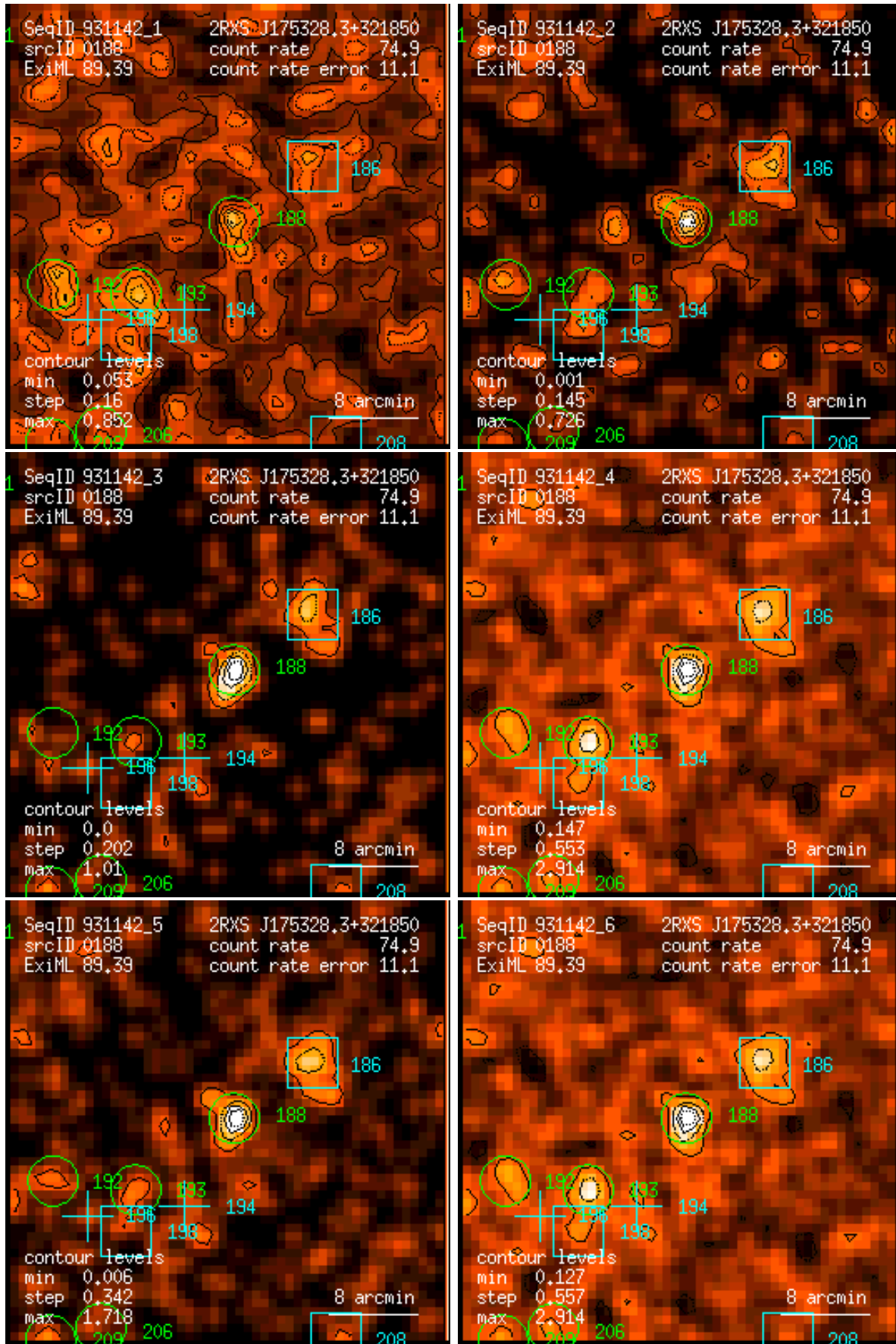
Figure 188: RASS 931142: detection 0188: band rate images, Gaussian filter: (1) PSPC channels 11 – 41, (2) 52 – 90, (3) 91 – 201, (4) 11 – 235, (5) 52 – 201, (6) 11 – 201. Broad band rates in counts/ks. Band rate contour levels in counts/ks/arcmin 2 .
