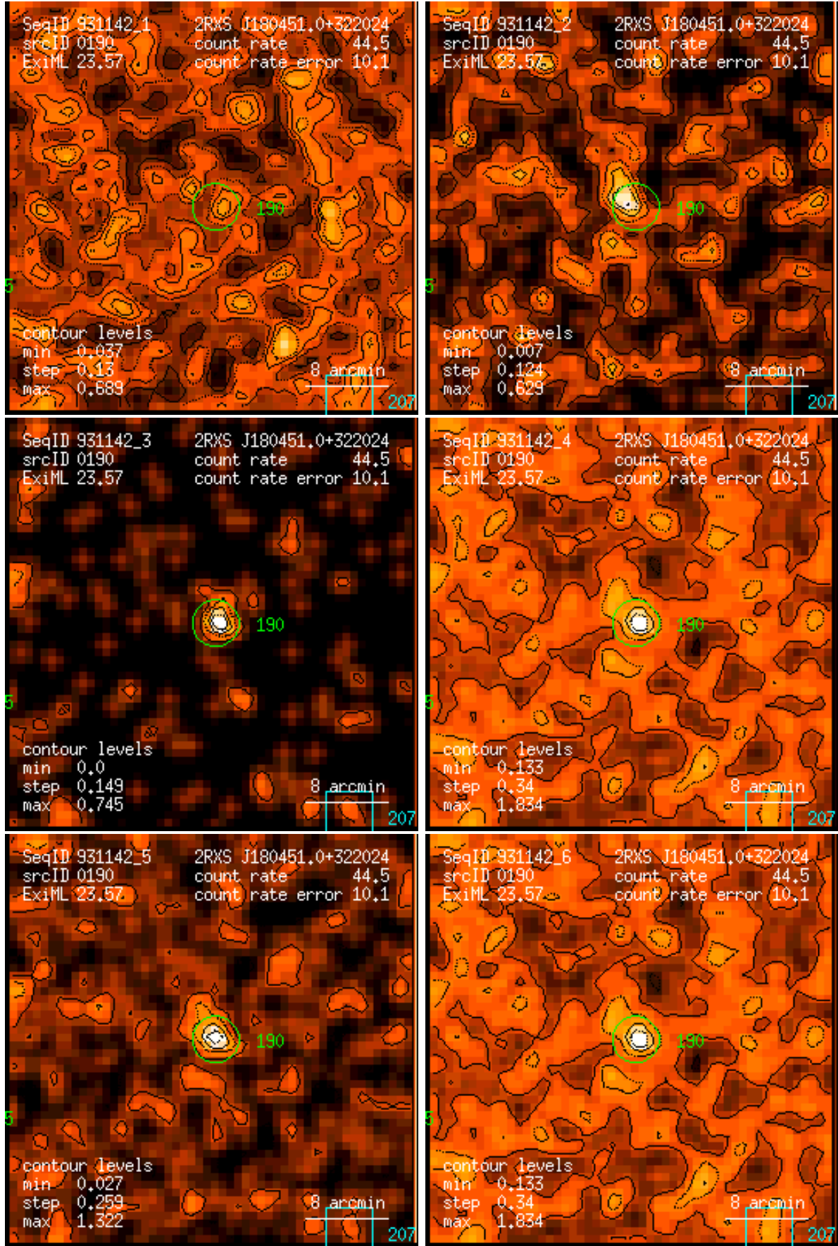
Figure 190: RASS 931142: detection 0190: band rate images, Gaussian filter: (1) PSPC channels 11 – 41, (2) 52 – 90, (3) 91 – 201, (4) 11 – 235, (5) 52 – 201, (6) 11 – 201. Broad band rates in counts/ks. Band rate contour levels in counts/ks/arcmin 2 .
