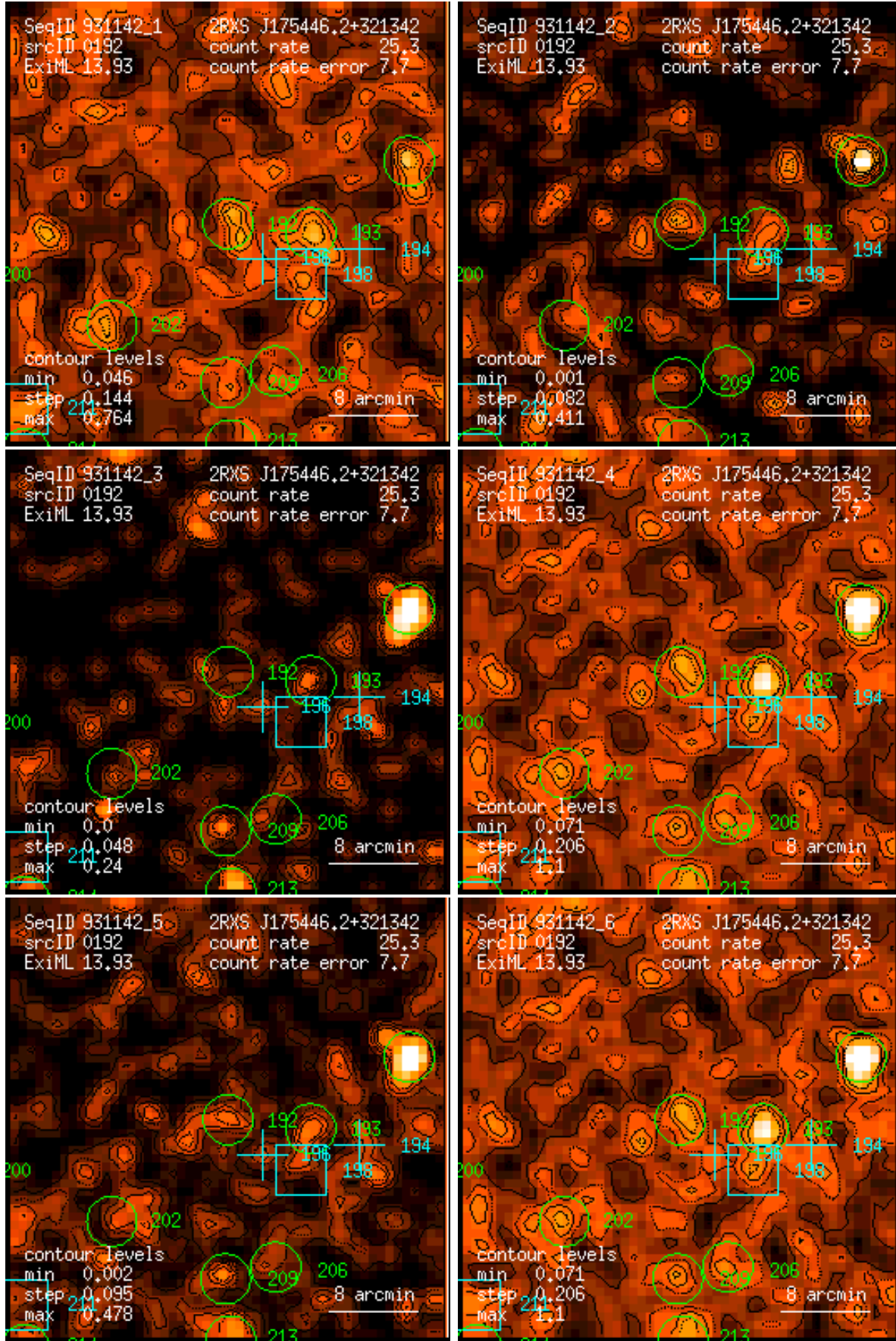
Figure 192: RASS 931142: detection 0192: band rate images, Gaussian filter: (1) PSPC channels 11 – 41, (2) 52 – 90, (3) 91 – 201, (4) 11 – 235, (5) 52 – 201, (6) 11 – 201. Broad band rates in counts/ks. Band rate contour levels in counts/ks/arcmin 2 .
