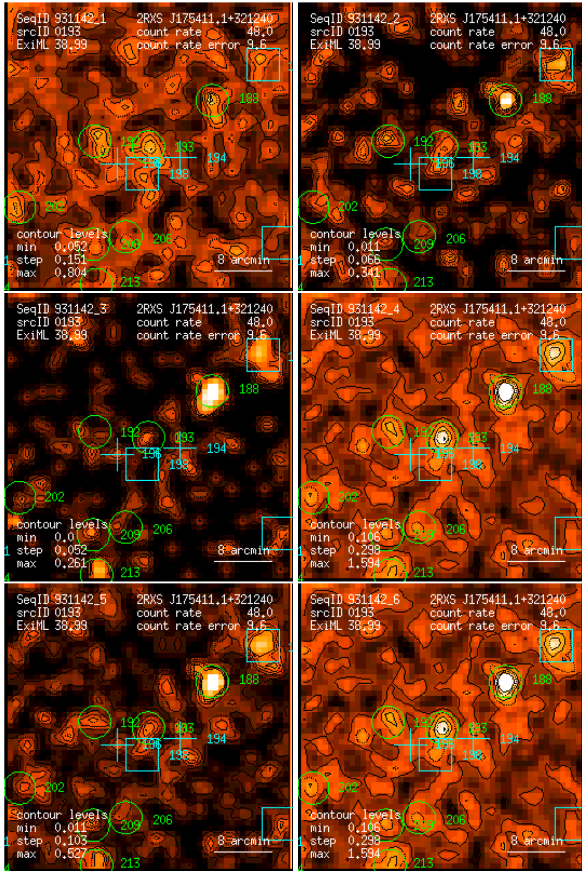
Figure 193: RASS 931142: detection 0193: band rate images, Gaussian filter: (1) PSPC channels 11 – 41, (2) 52 – 90, (3) 91 – 201, (4) 11 – 235, (5) 52 – 201, (6) 11 – 201. Broad band rates in counts/ks. Band rate contour levels in counts/ks/arcmin 2 .
