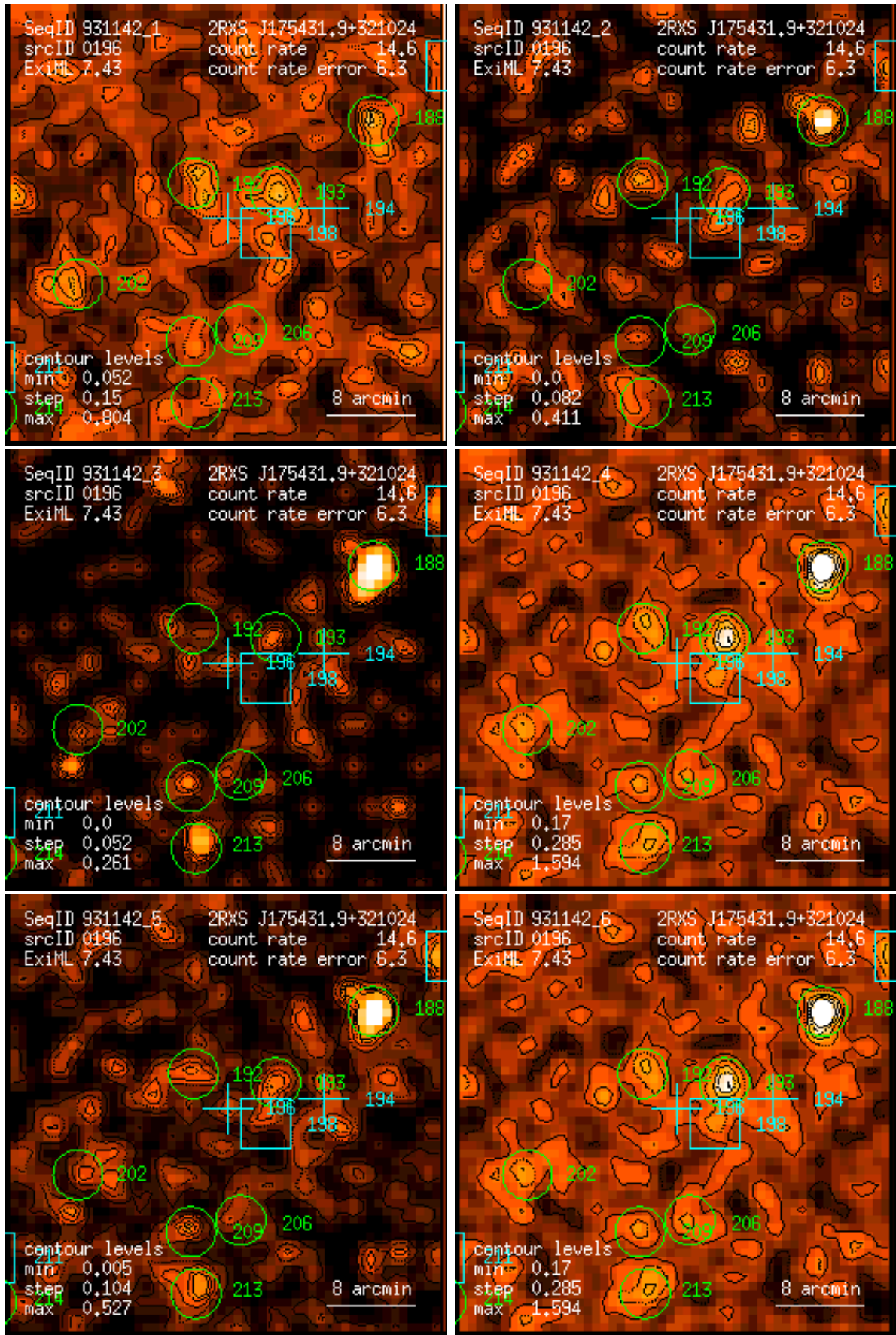
Figure 196: RASS 931142: detection 0196: band rate images, Gaussian filter: (1) PSPC channels 11 – 41, (2) 52 – 90, (3) 91 – 201, (4) 11 – 235, (5) 52 – 201, (6) 11 – 201. Broad band rates in counts/ks. Band rate contour levels in counts/ks/arcmin 2 .
