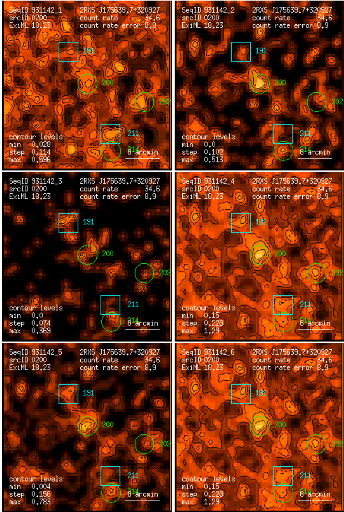
Figure 200: RASS 931142: detection 0200: band rate images, Gaussian filter: (1) PSPC channels 11 – 41, (2) 52 – 90, (3) 91 – 201, (4) 11 – 235, (5) 52 – 201, (6) 11 – 201. Broad band rates in counts/ks. Band rate contour levels in counts/ks/arcmin 2 .
