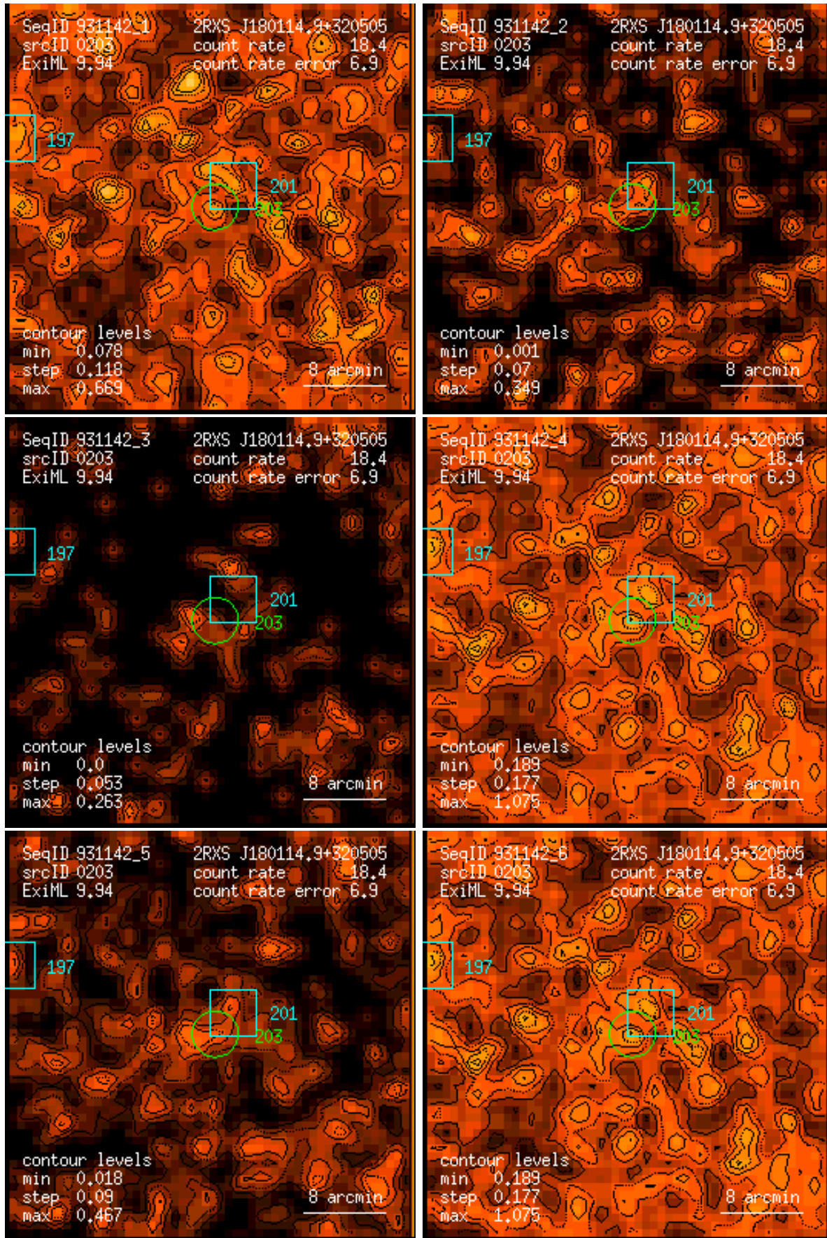
Figure 203: RASS 931142: detection 0203: band rate images, Gaussian filter: (1) PSPC channels 11 – 41, (2) 52 – 90, (3) 91 – 201, (4) 11 – 235, (5) 52 – 201, (6) 11 – 201. Broad band rates in counts/ks. Band rate contour levels in counts/ks/arcmin 2 .
