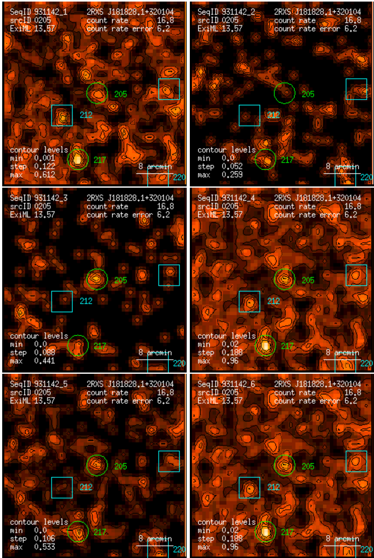
Figure 205: RASS 931142: detection 0205: band rate images, Gaussian filter: (1) PSPC channels 11 – 41, (2) 52 – 90, (3) 91 – 201, (4) 11 – 235, (5) 52 – 201, (6) 11 – 201. Broad band rates in counts/ks. Band rate contour levels in counts/ks/arcmin 2 .
