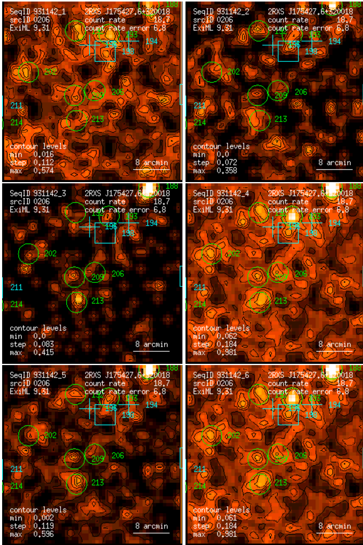
Figure 206: RASS 931142: detection 0206: band rate images, Gaussian filter: (1) PSPC channels 11 – 41, (2) 52 – 90, (3) 91 – 201, (4) 11 – 235, (5) 52 – 201, (6) 11 – 201. Broad band rates in counts/ks. Band rate contour levels in counts/ks/arcmin 2 .
