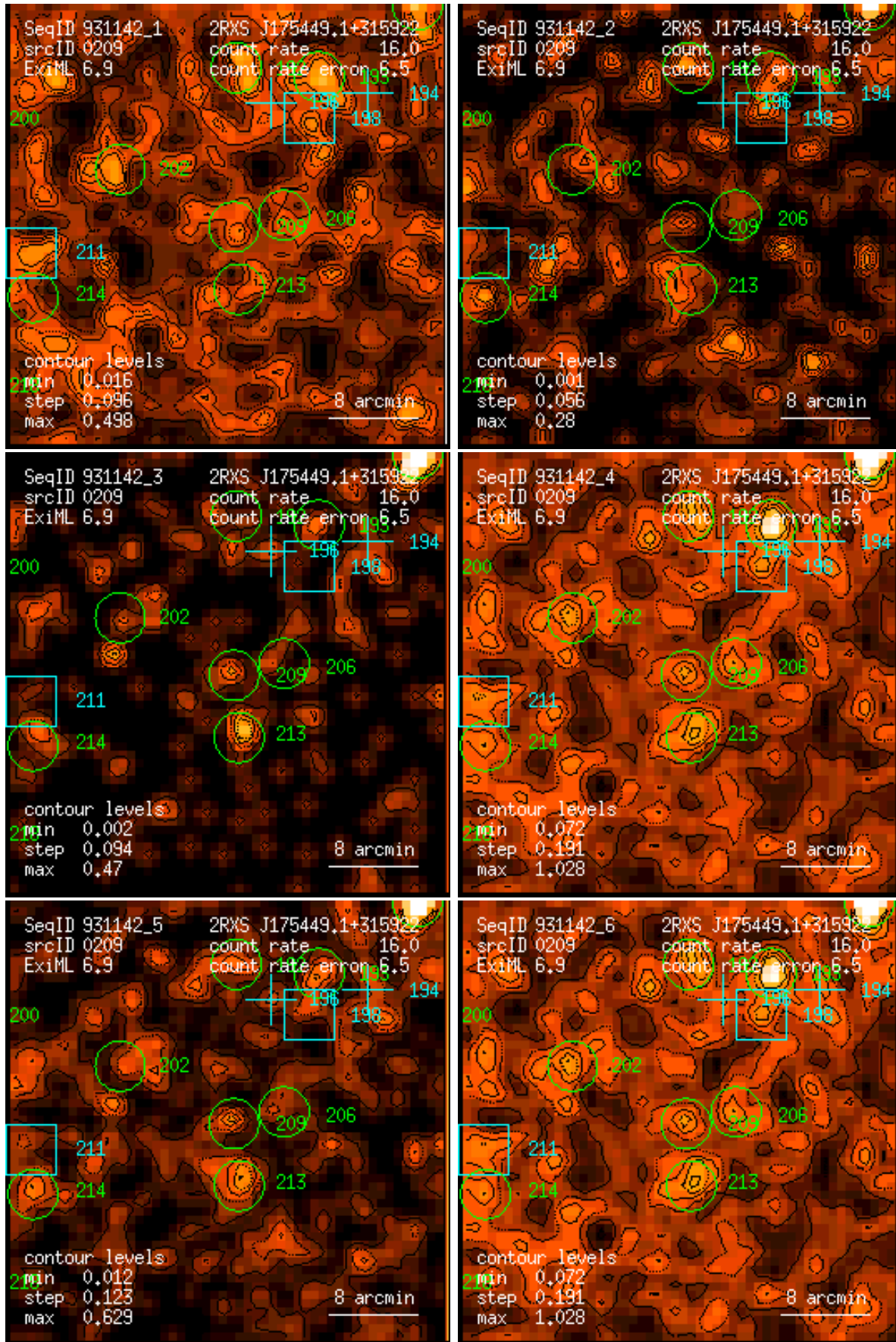
Figure 209: RASS 931142: detection 0209: band rate images, Gaussian filter: (1) PSPC channels 11 – 41, (2) 52 – 90, (3) 91 – 201, (4) 11 – 235, (5) 52 – 201, (6) 11 – 201. Broad band rates in counts/ks. Band rate contour levels in counts/ks/arcmin 2 .
