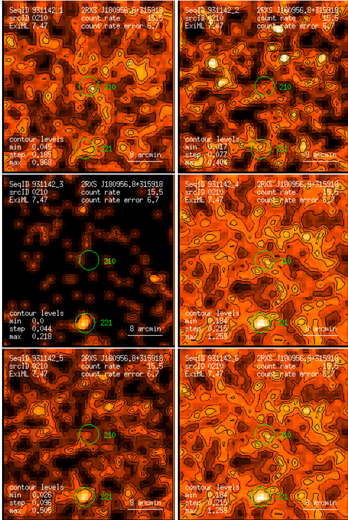
Figure 210: RASS 931142: detection 0210: band rate images, Gaussian filter: (1) PSPC channels 11 – 41, (2) 52 – 90, (3) 91 – 201, (4) 11 – 235, (5) 52 – 201, (6) 11 – 201. Broad band rates in counts/ks. Band rate contour levels in counts/ks/arcmin 2 .
