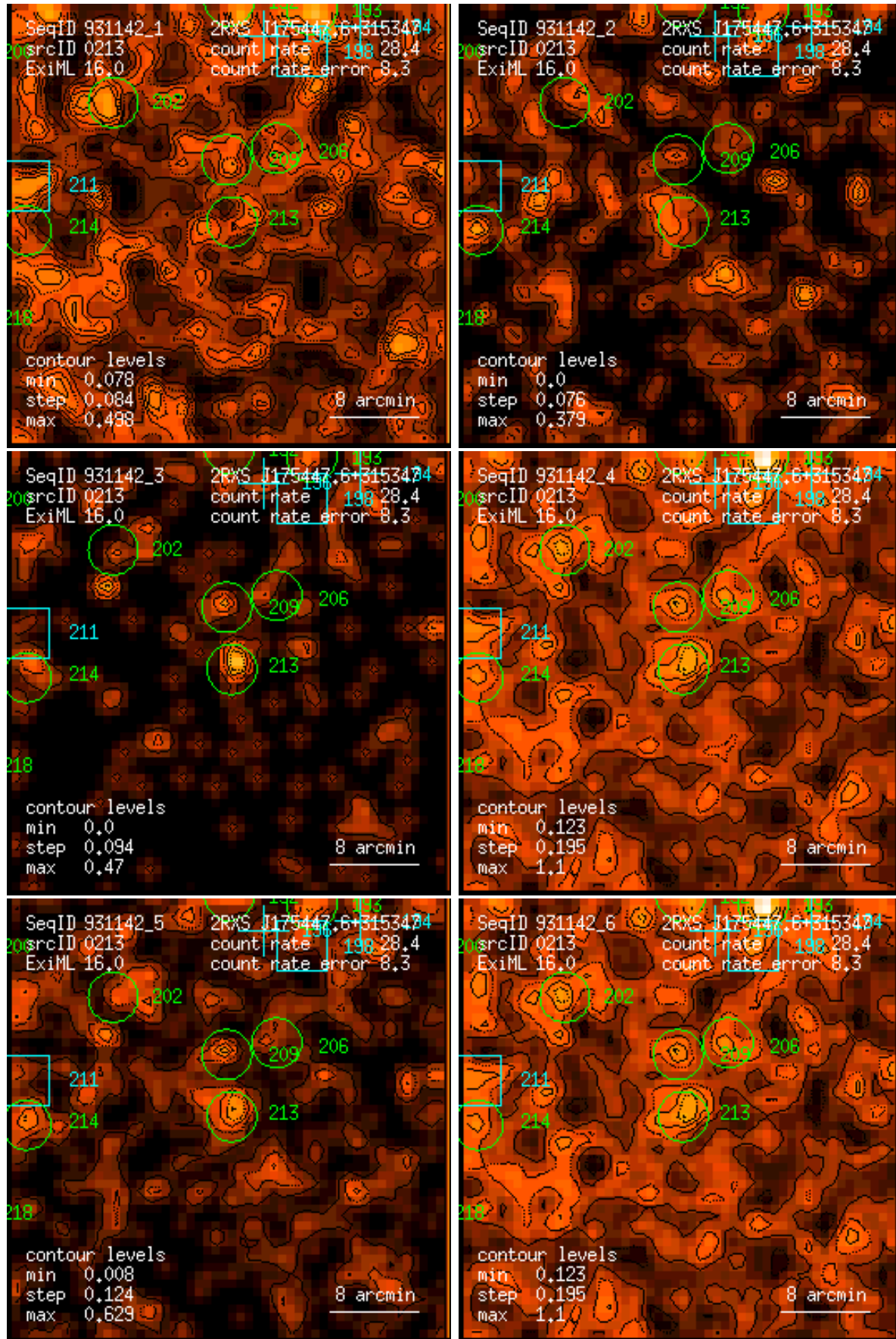
Figure 213: RASS 931142: detection 0213: band rate images, Gaussian filter: (1) PSPC channels 11 – 41, (2) 52 – 90, (3) 91 – 201, (4) 11 – 235, (5) 52 – 201, (6) 11 – 201. Broad band rates in counts/ks. Band rate contour levels in counts/ks/arcmin 2 .
