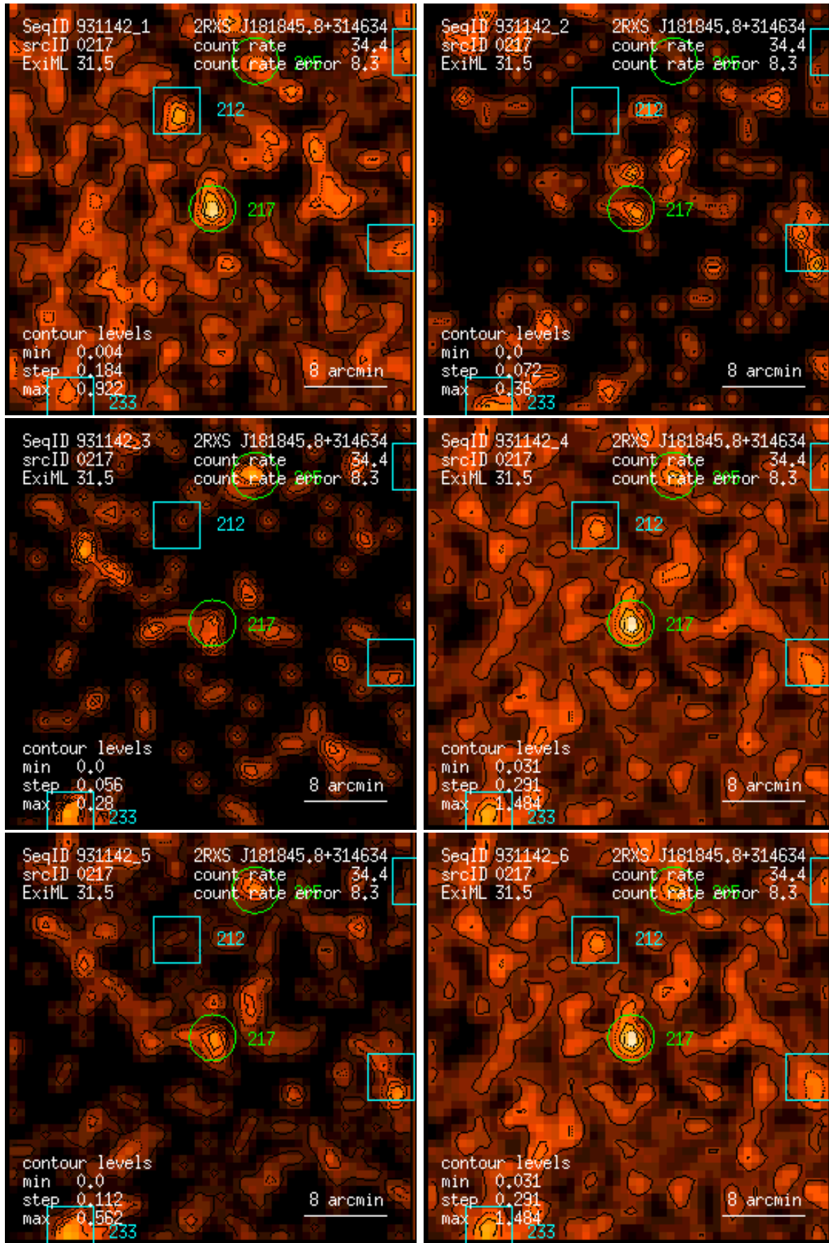
Figure 217: RASS 931142: detection 0217: band rate images, Gaussian filter: (1) PSPC channels 11 – 41, (2) 52 – 90, (3) 91 – 201, (4) 11 – 235, (5) 52 – 201, (6) 11 – 201. Broad band rates in counts/ks. Band rate contour levels in counts/ks/arcmin 2 .
