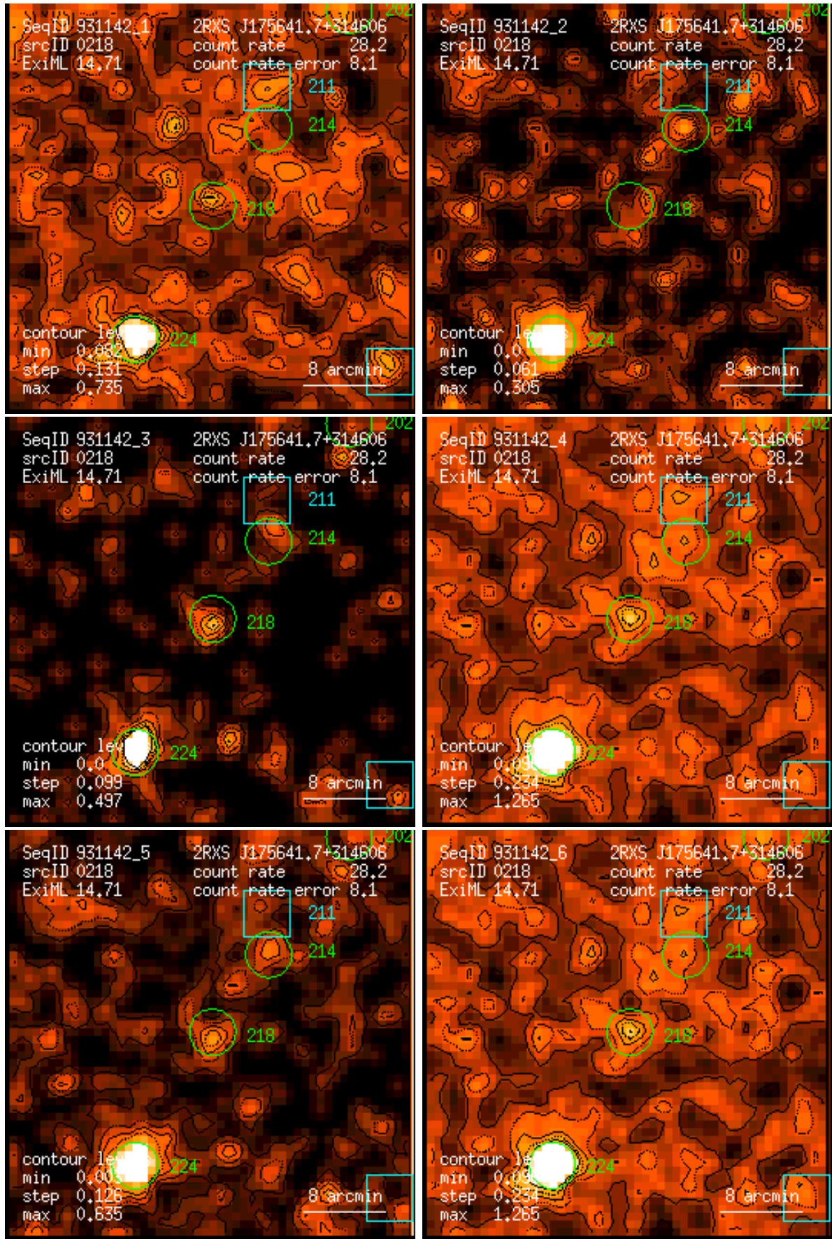
Figure 218: RASS 931142: detection 0218: band rate images, Gaussian filter: (1) PSPC channels 11 – 41, (2) 52 – 90, (3) 91 – 201, (4) 11 – 235, (5) 52 – 201, (6) 11 – 201. Broad band rates in counts/ks. Band rate contour levels in counts/ks/arcmin 2 .
