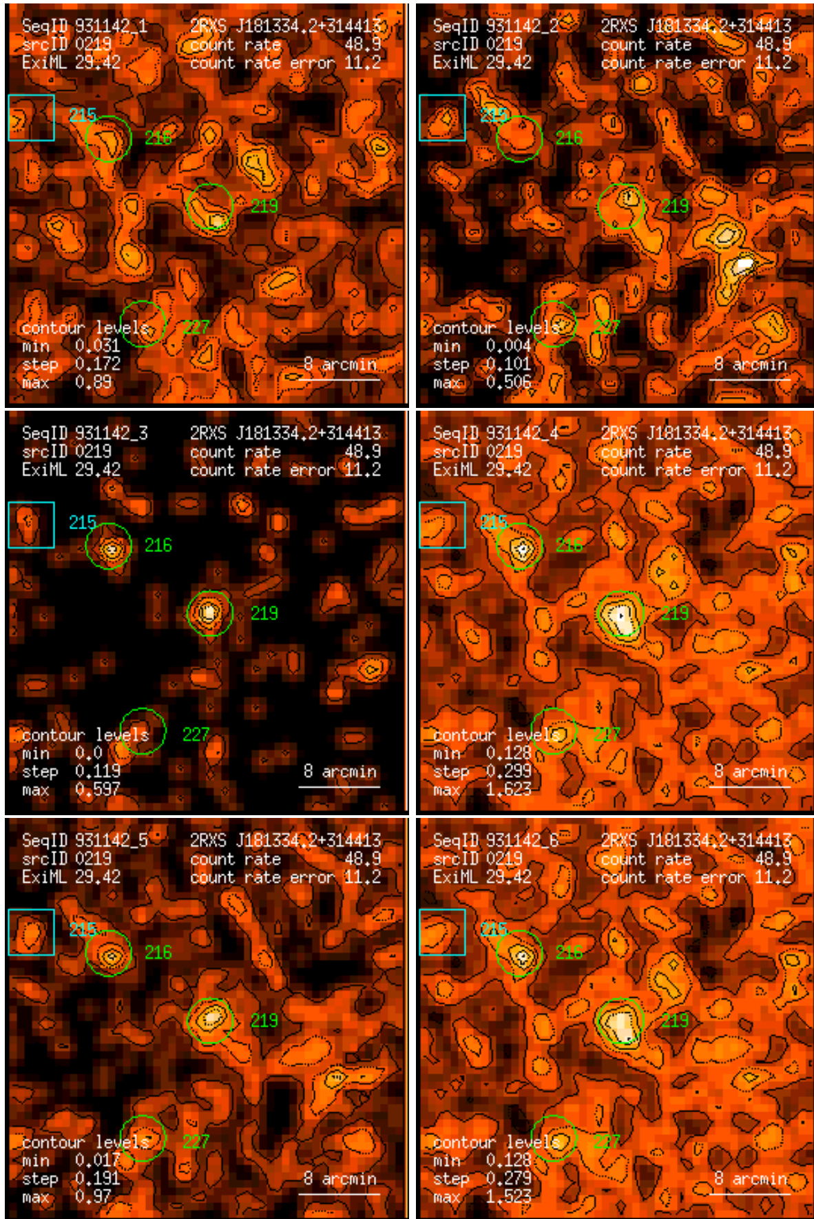
Figure 219: RASS 931142: detection 0219: band rate images, Gaussian filter: (1) PSPC channels 11 – 41, (2) 52 – 90, (3) 91 – 201, (4) 11 – 235, (5) 52 – 201, (6) 11 – 201. Broad band rates in counts/ks. Band rate contour levels in counts/ks/arcmin 2 .
