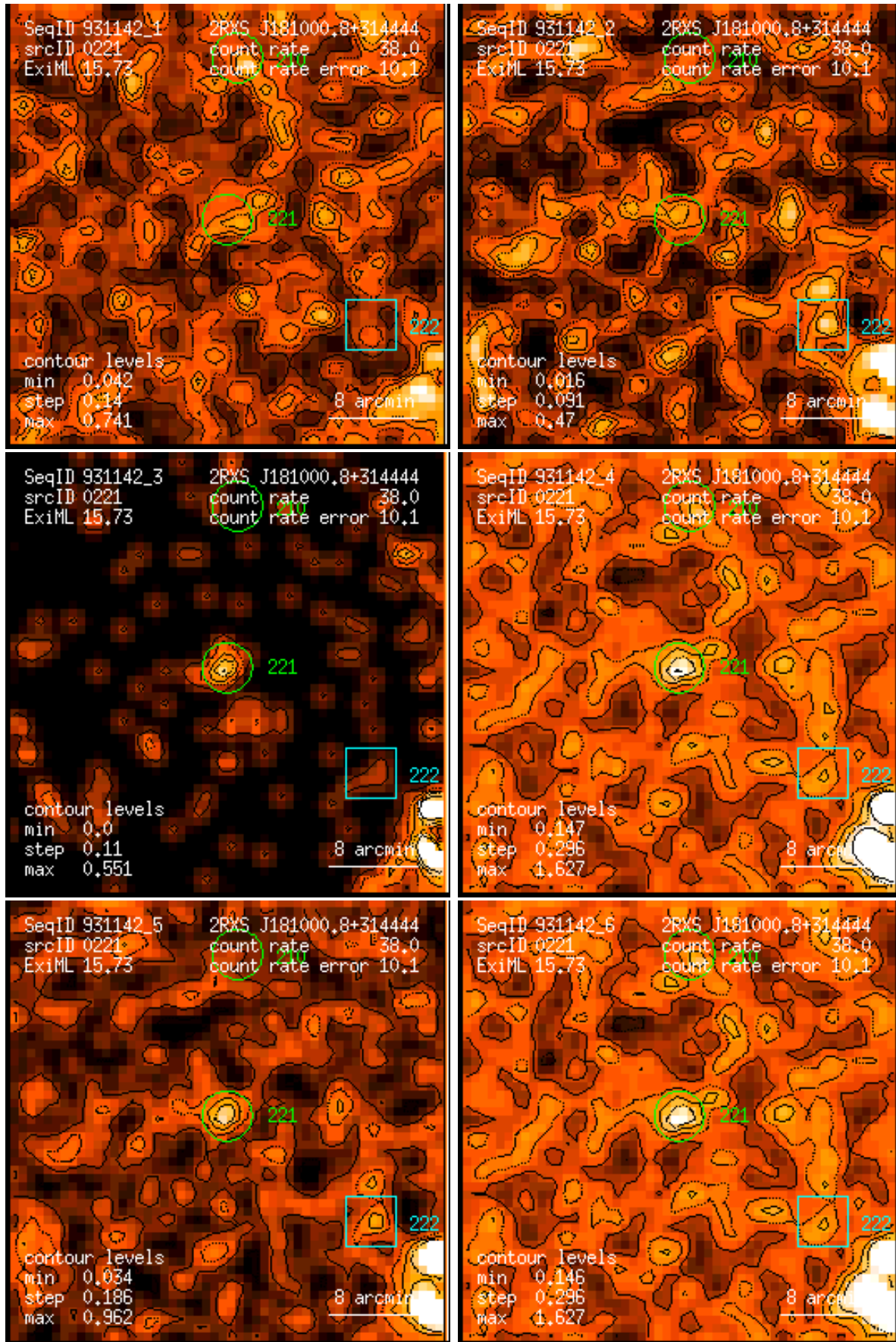
Figure 221: RASS 931142: detection 0221: band rate images, Gaussian filter: (1) PSPC channels 11 – 41, (2) 52 – 90, (3) 91 – 201, (4) 11 – 235, (5) 52 – 201, (6) 11 – 201. Broad band rates in counts/ks. Band rate contour levels in counts/ks/arcmin 2 .
