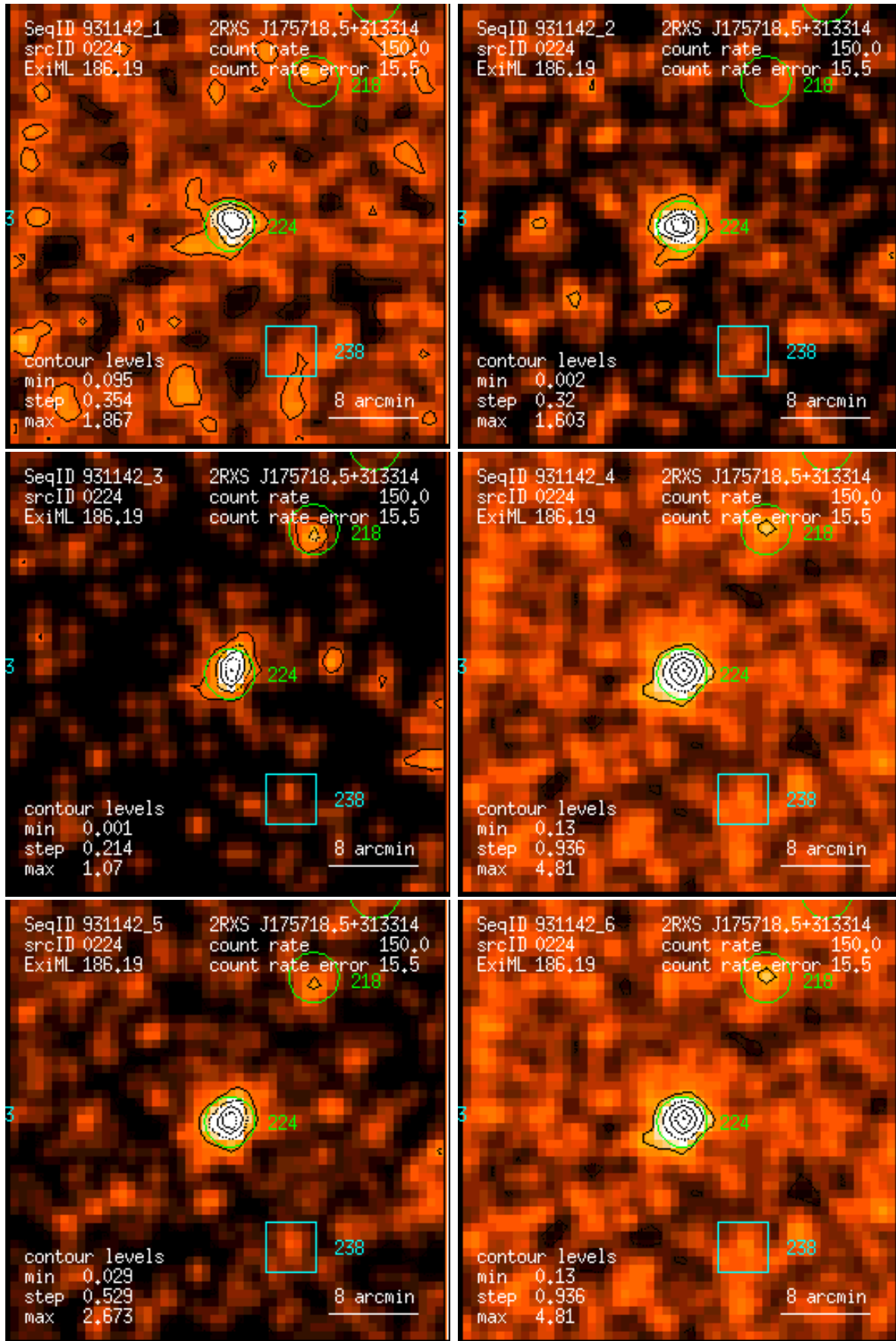
Figure 224: RASS 931142: detection 0224: band rate images, Gaussian filter: (1) PSPC channels 11 – 41, (2) 52 – 90, (3) 91 – 201, (4) 11 – 235, (5) 52 – 201, (6) 11 – 201. Broad band rates in counts/ks. Band rate contour levels in counts/ks/arcmin 2 .
