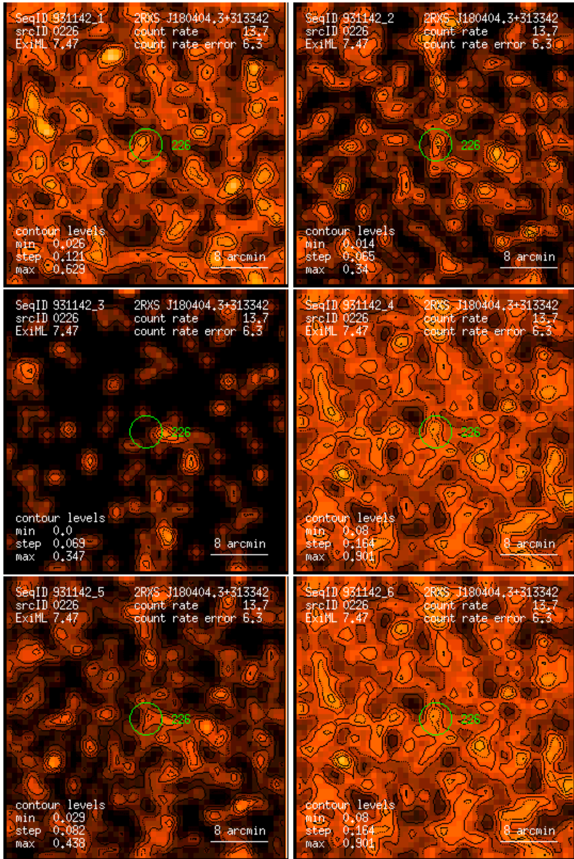
Figure 226: RASS 931142: detection 0226: band rate images, Gaussian filter: (1) PSPC channels 11 – 41, (2) 52 – 90, (3) 91 – 201, (4) 11 – 235, (5) 52 – 201, (6) 11 – 201. Broad band rates in counts/ks. Band rate contour levels in counts/ks/arcmin 2 .
