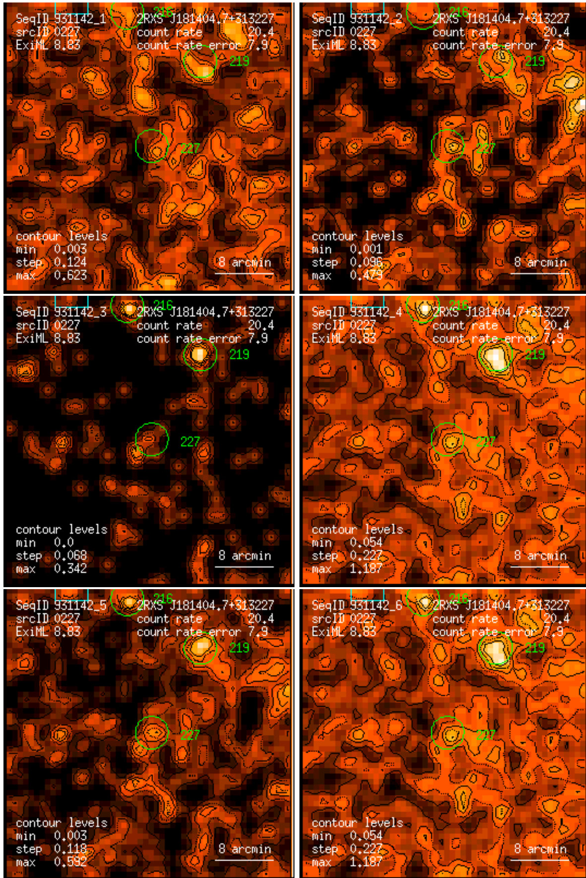
Figure 227: RASS 931142: detection 0227: band rate images, Gaussian filter: (1) PSPC channels 11 – 41, (2) 52 – 90, (3) 91 – 201, (4) 11 – 235, (5) 52 – 201, (6) 11 – 201. Broad band rates in counts/ks. Band rate contour levels in counts/ks/arcmin 2 .
