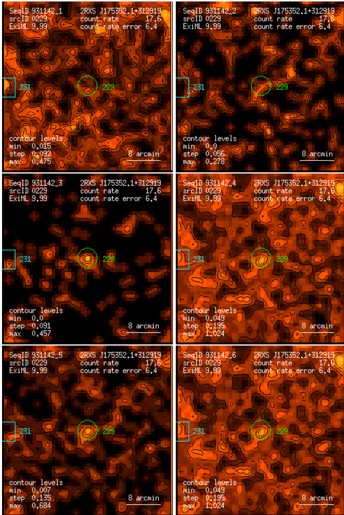
Figure 229: RASS 931142: detection 0229: band rate images, Gaussian filter: (1) PSPC channels 11 – 41, (2) 52 – 90, (3) 91 – 201, (4) 11 – 235, (5) 52 – 201, (6) 11 – 201. Broad band rates in counts/ks. Band rate contour levels in counts/ks/arcmin 2 .
