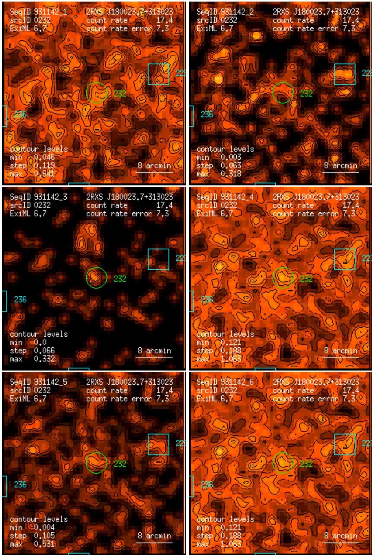
Figure 232: RASS 931142: detection 0232: band rate images, Gaussian filter: (1) PSPC channels 11 – 41, (2) 52 – 90, (3) 91 – 201, (4) 11 – 235, (5) 52 – 201, (6) 11 – 201. Broad band rates in counts/ks. Band rate contour levels in counts/ks/arcmin 2 .
