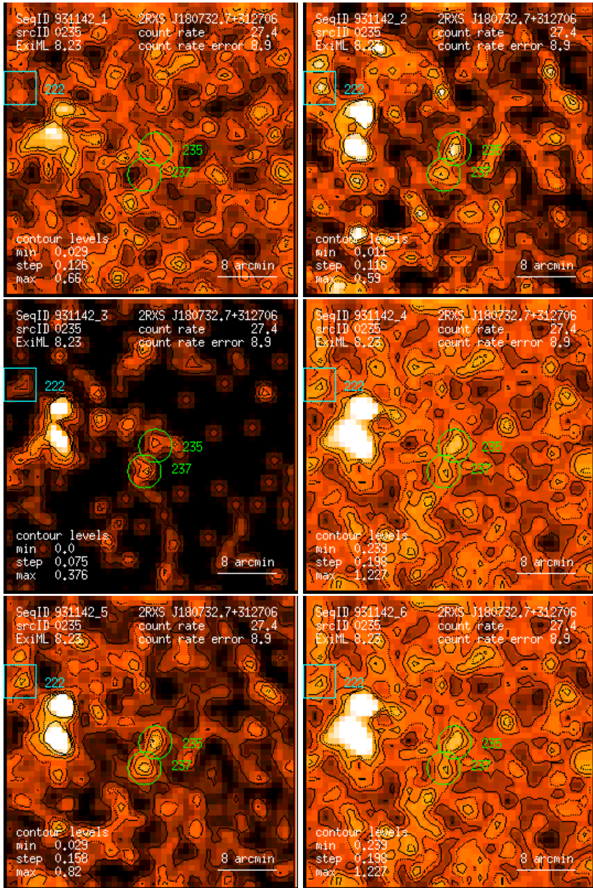
Figure 235: RASS 931142: detection 0235: band rate images, Gaussian filter: (1) PSPC channels 11 – 41, (2) 52 – 90, (3) 91 – 201, (4) 11 – 235, (5) 52 – 201, (6) 11 – 201. Broad band rates in counts/ks. Band rate contour levels in counts/ks/arcmin 2 .
