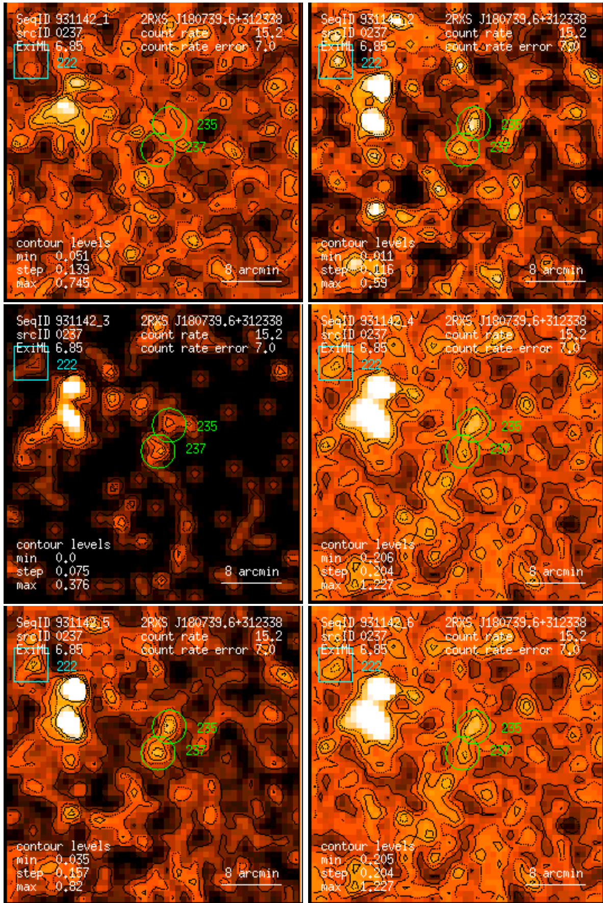
Figure 237: RASS 931142: detection 0237: band rate images, Gaussian filter: (1) PSPC channels 11 – 41, (2) 52 – 90, (3) 91 – 201, (4) 11 – 235, (5) 52 – 201, (6) 11 – 201. Broad band rates in counts/ks. Band rate contour levels in counts/ks/arcmin 2 .
