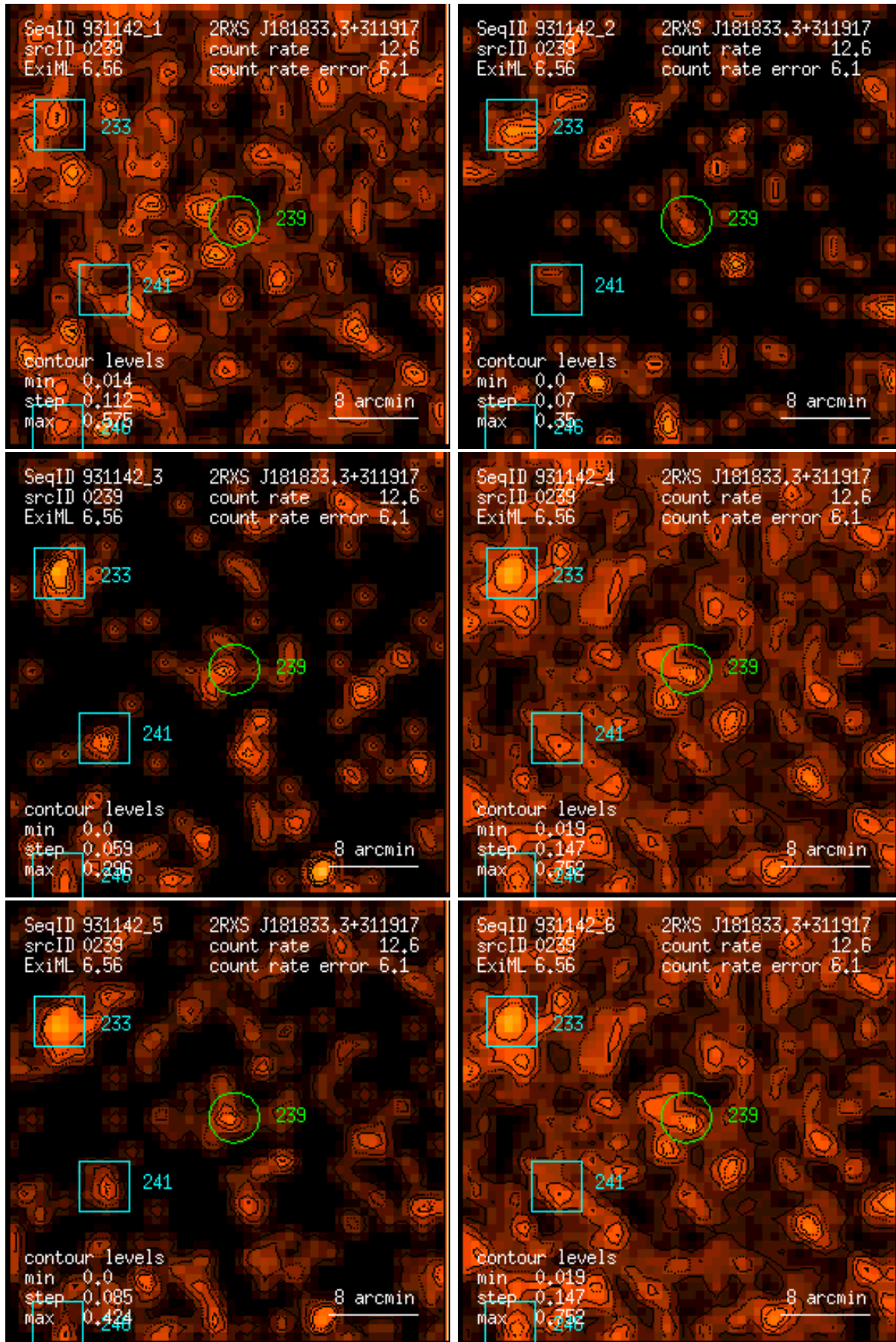
Figure 239: RASS 931142: detection 0239: band rate images, Gaussian filter: (1) PSPC channels 11 – 41, (2) 52 – 90, (3) 91 – 201, (4) 11 – 235, (5) 52 – 201, (6) 11 – 201. Broad band rates in counts/ks. Band rate contour levels in counts/ks/arcmin 2 .
