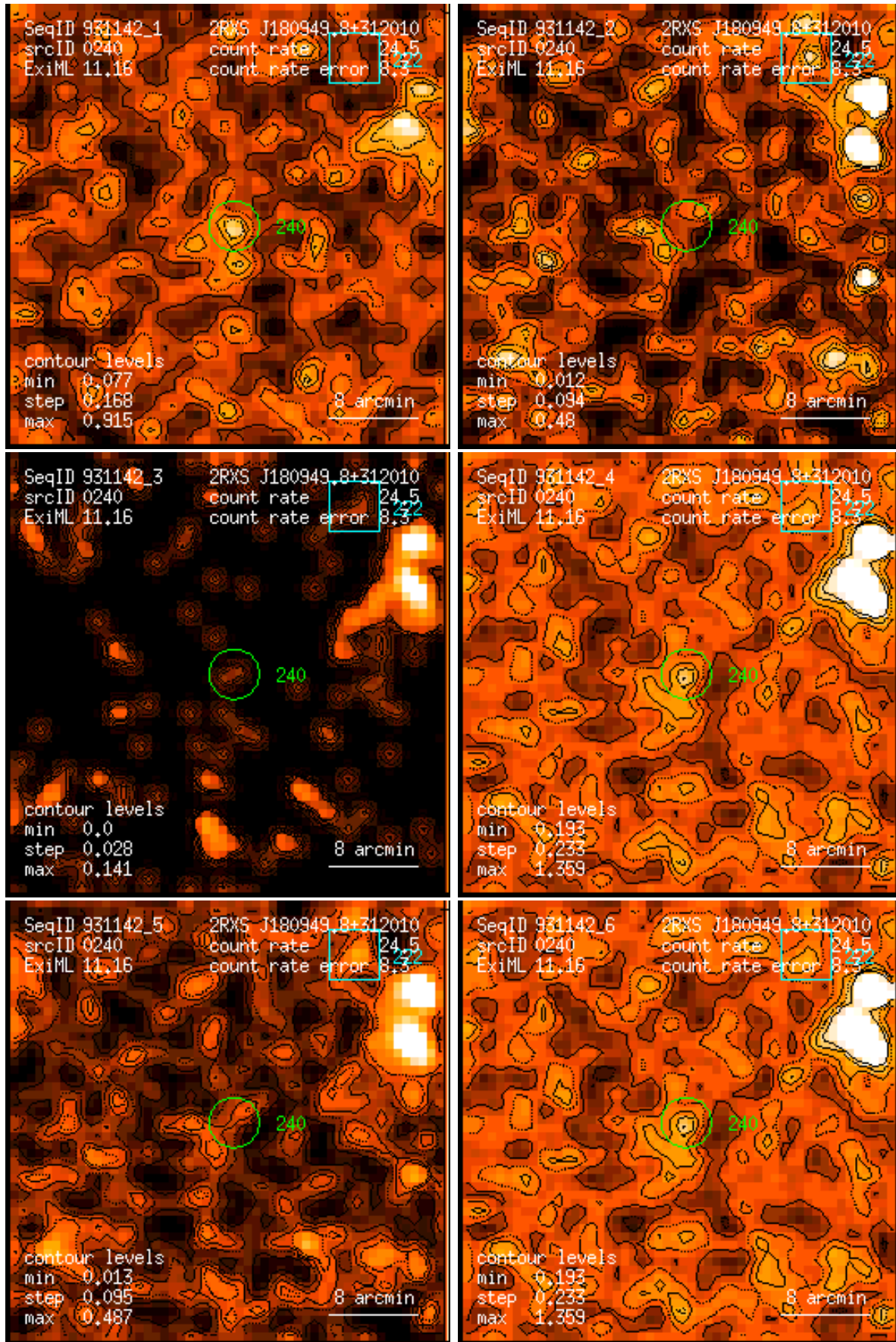
Figure 240: RASS 931142: detection 0240: band rate images, Gaussian filter: (1) PSPC channels 11 – 41, (2) 52 – 90, (3) 91 – 201, (4) 11 – 235, (5) 52 – 201, (6) 11 – 201. Broad band rates in counts/ks. Band rate contour levels in counts/ks/arcmin 2 .
