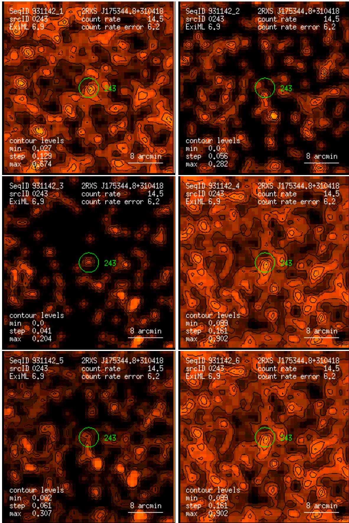
Figure 243: RASS 931142: detection 0243: band rate images, Gaussian filter: (1) PSPC channels 11 – 41, (2) 52 – 90, (3) 91 – 201, (4) 11 – 235, (5) 52 – 201, (6) 11 – 201. Broad band rates in counts/ks. Band rate contour levels in counts/ks/arcmin 2 .
