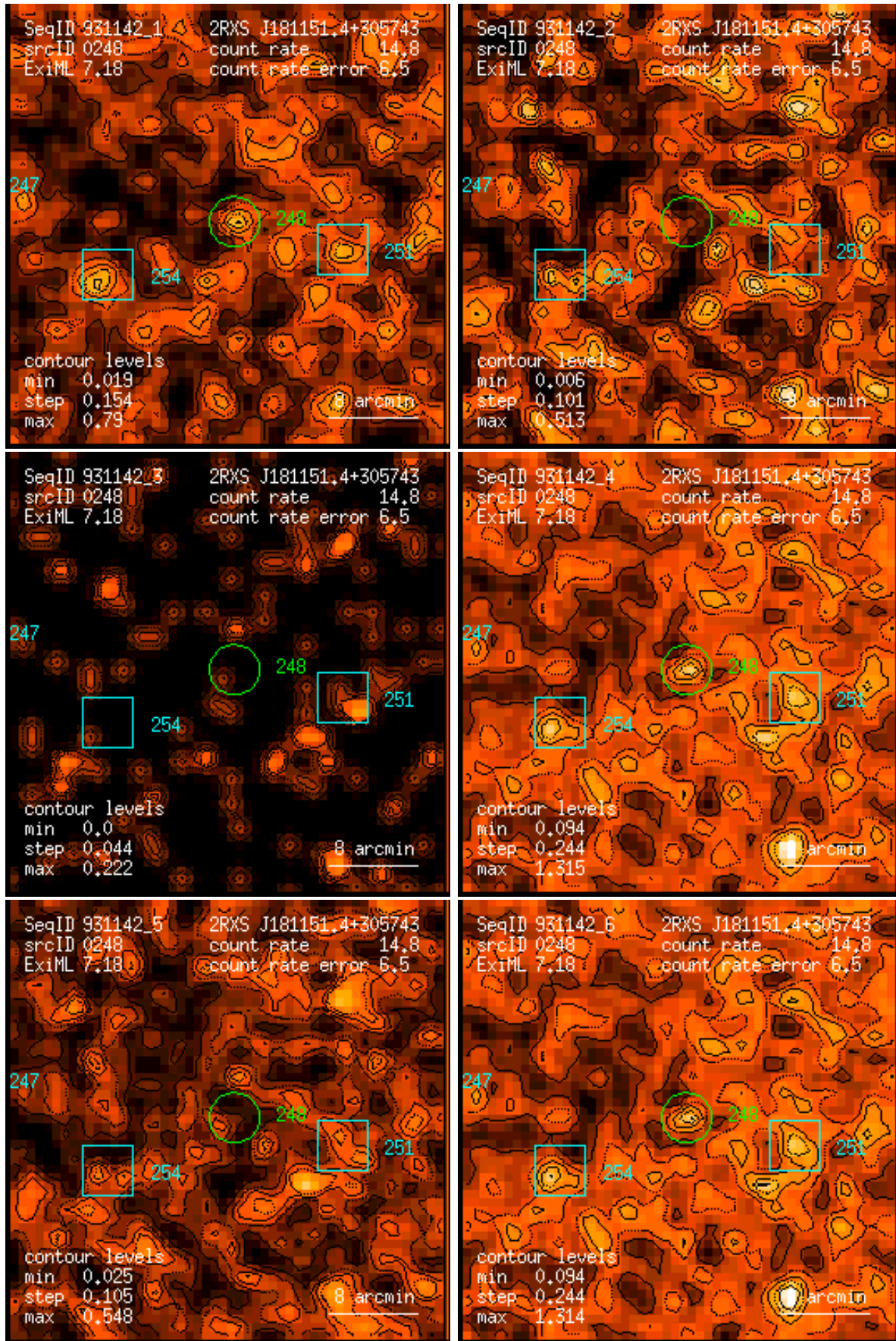
Figure 248: RASS 931142: detection 0248: band rate images, Gaussian filter: (1) PSPC channels 11 – 41, (2) 52 – 90, (3) 91 – 201, (4) 11 – 235, (5) 52 – 201, (6) 11 – 201. Broad band rates in counts/ks. Band rate contour levels in counts/ks/arcmin 2 .
