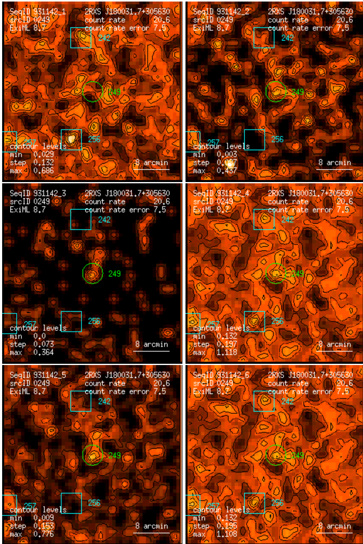
Figure 249: RASS 931142: detection 0249: band rate images, Gaussian filter: (1) PSPC channels 11 – 41, (2) 52 – 90, (3) 91 – 201, (4) 11 – 235, (5) 52 – 201, (6) 11 – 201. Broad band rates in counts/ks. Band rate contour levels in counts/ks/arcmin 2 .
