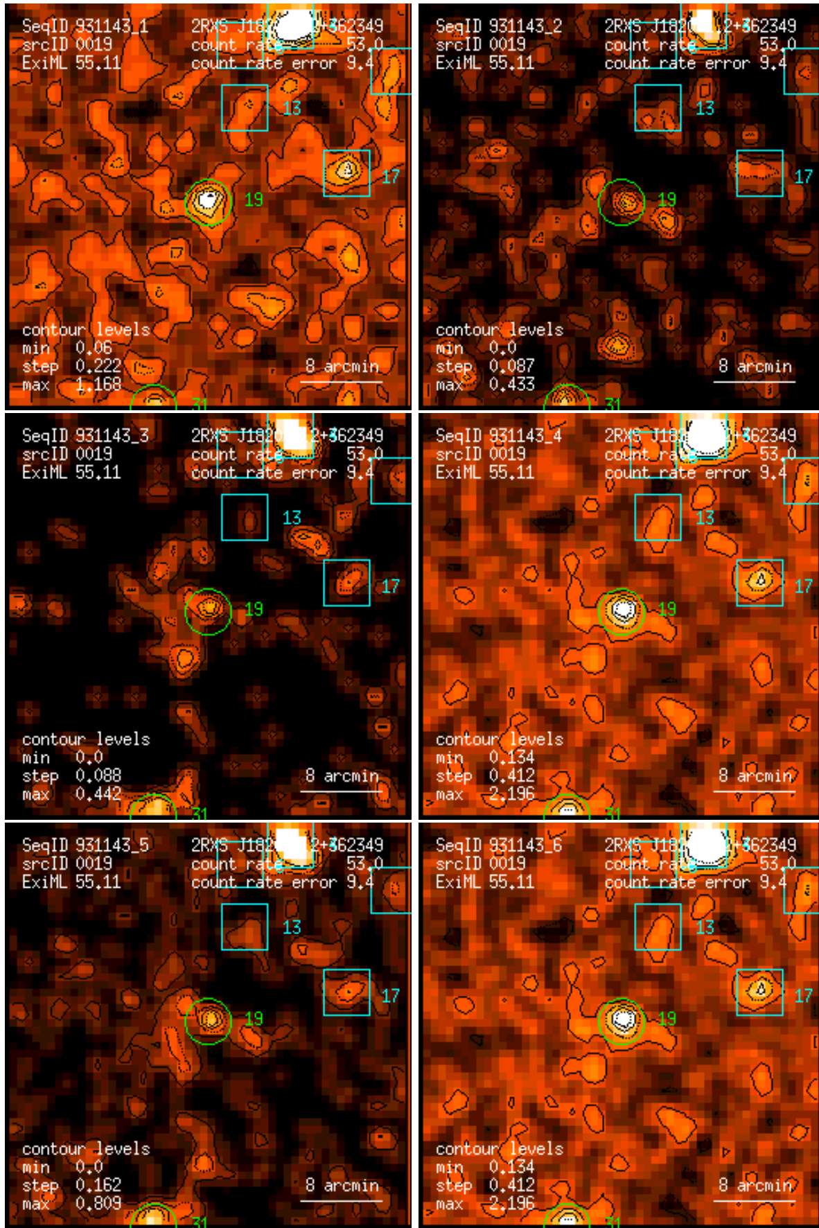
Figure 19: RASS 931143: detection 0019: band rate images, Gaussian filter: (1) PSPC channels 11 – 41, (2) 52 – 90, (3) 91 – 201, (4) 11 – 235, (5) 52 – 201, (6) 11 – 201. Broad band rates in counts/ks. Band rate contour levels in counts/ks/arcmin 2 .
