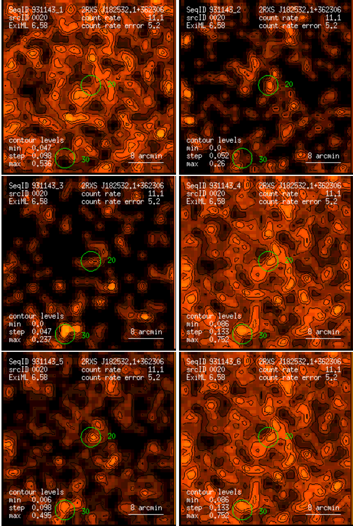
Figure 20: RASS 931143: detection 0020: band rate images, Gaussian filter: (1) PSPC channels 11 – 41, (2) 52 – 90, (3) 91 – 201, (4) 11 – 235, (5) 52 – 201, (6) 11 – 201. Broad band rates in counts/ks. Band rate contour levels in counts/ks/arcmin 2 .
