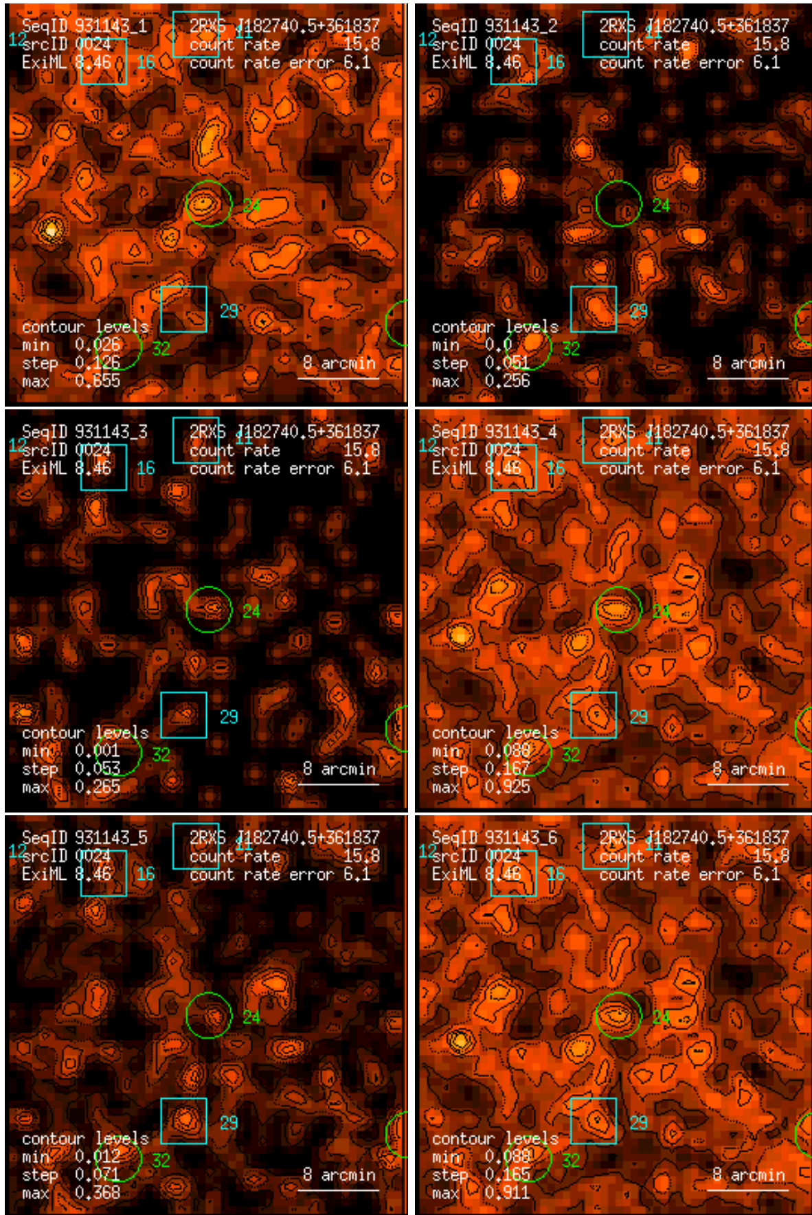
Figure 24: RASS 931143: detection 0024: band rate images, Gaussian filter: (1) PSPC channels 11 – 41, (2) 52 – 90, (3) 91 – 201, (4) 11 – 235, (5) 52 – 201, (6) 11 – 201. Broad band rates in counts/ks. Band rate contour levels in counts/ks/arcmin 2 .
