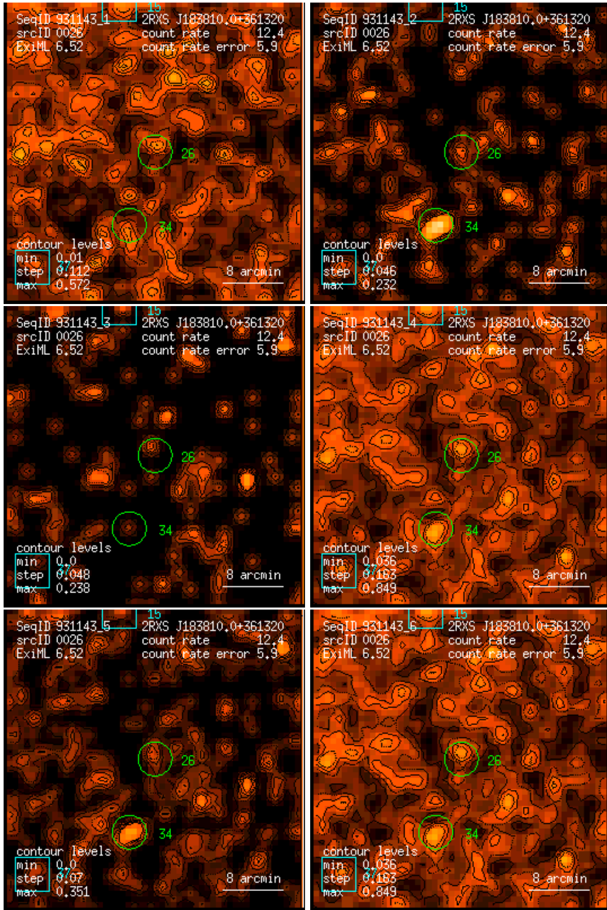
Figure 26: RASS 931143: detection 0026: band rate images, Gaussian filter: (1) PSPC channels 11 – 41, (2) 52 – 90, (3) 91 – 201, (4) 11 – 235, (5) 52 – 201, (6) 11 – 201. Broad band rates in counts/ks. Band rate contour levels in counts/ks/arcmin 2 .
