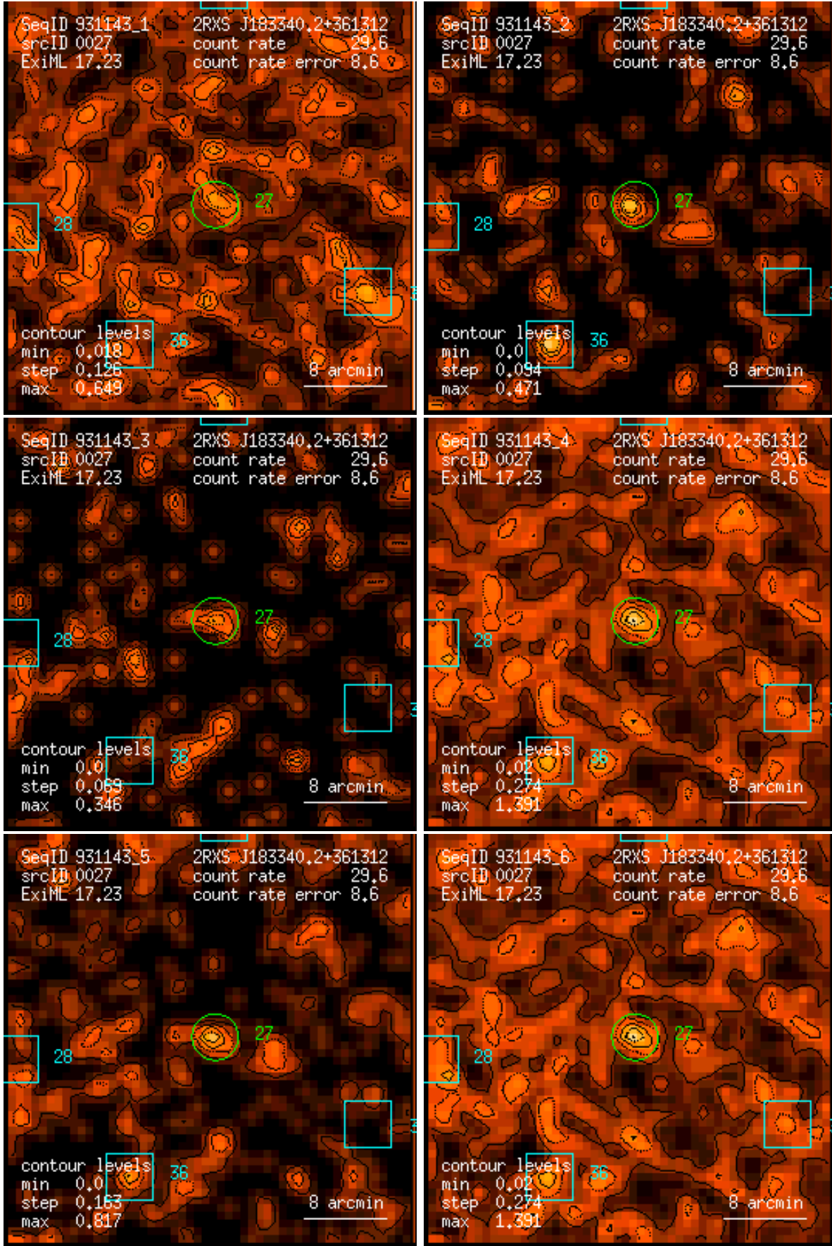
Figure 27: RASS 931143: detection 0027: band rate images, Gaussian filter: (1) PSPC channels 11 – 41, (2) 52 – 90, (3) 91 – 201, (4) 11 – 235, (5) 52 – 201, (6) 11 – 201. Broad band rates in counts/ks. Band rate contour levels in counts/ks/arcmin 2 .
