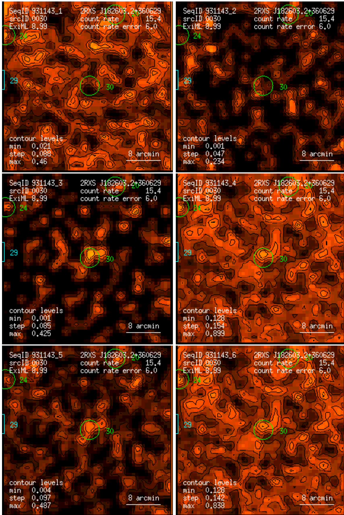
Figure 30: RASS 931143: detection 0030: band rate images, Gaussian filter: (1) PSPC channels 11 – 41, (2) 52 – 90, (3) 91 – 201, (4) 11 – 235, (5) 52 – 201, (6) 11 – 201. Broad band rates in counts/ks. Band rate contour levels in counts/ks/arcmin 2 .
