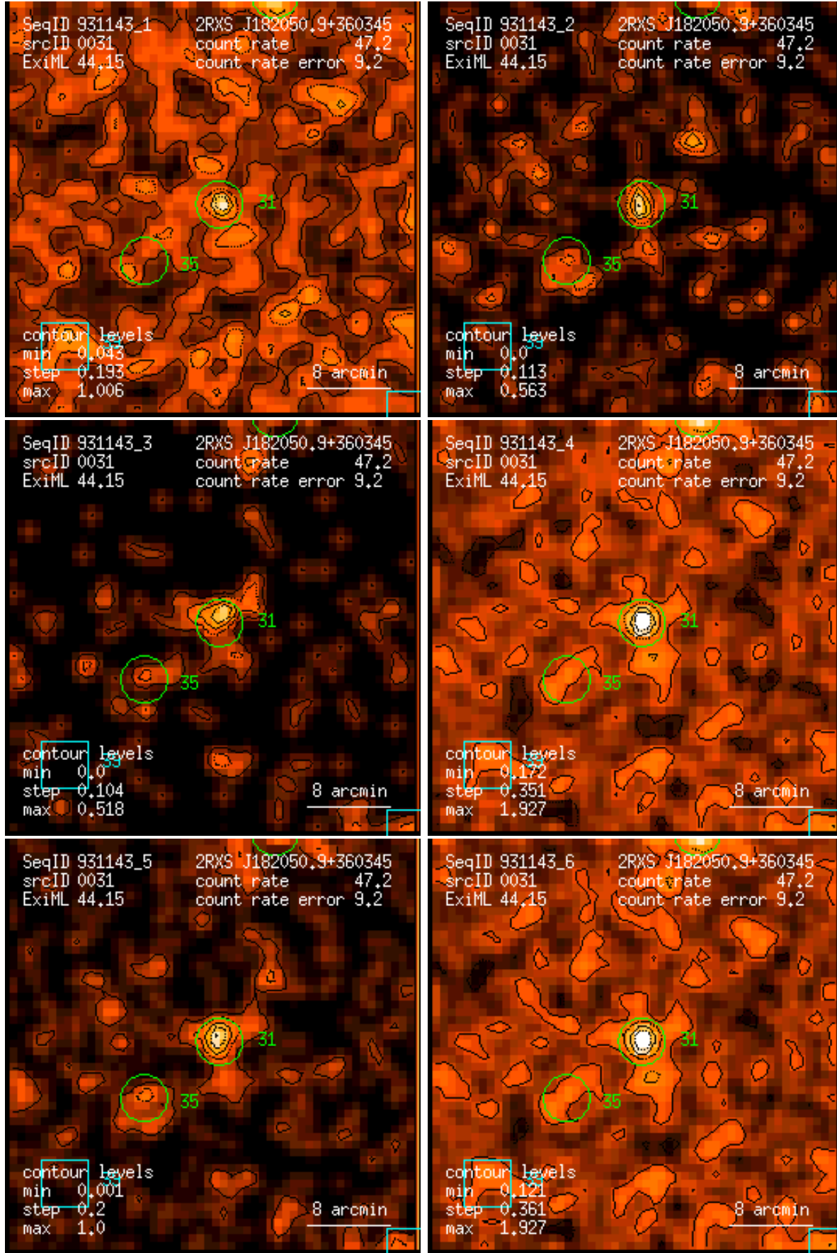
Figure 31: RASS 931143: detection 0031: band rate images, Gaussian filter: (1) PSPC channels 11 – 41, (2) 52 – 90, (3) 91 – 201, (4) 11 – 235, (5) 52 – 201, (6) 11 – 201. Broad band rates in counts/ks. Band rate contour levels in counts/ks/arcmin 2 .
