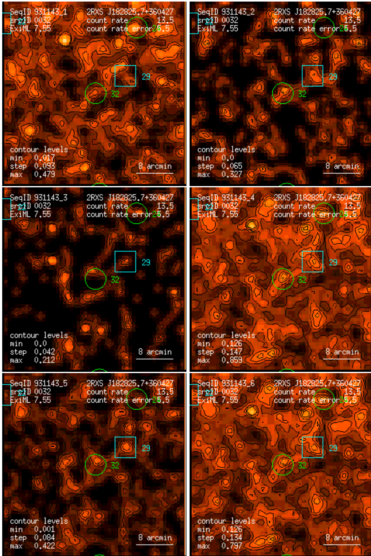
Figure 32: RASS 931143: detection 0032: band rate images, Gaussian filter: (1) PSPC channels 11 – 41, (2) 52 – 90, (3) 91 – 201, (4) 11 – 235, (5) 52 – 201, (6) 11 – 201. Broad band rates in counts/ks. Band rate contour levels in counts/ks/arcmin 2 .
