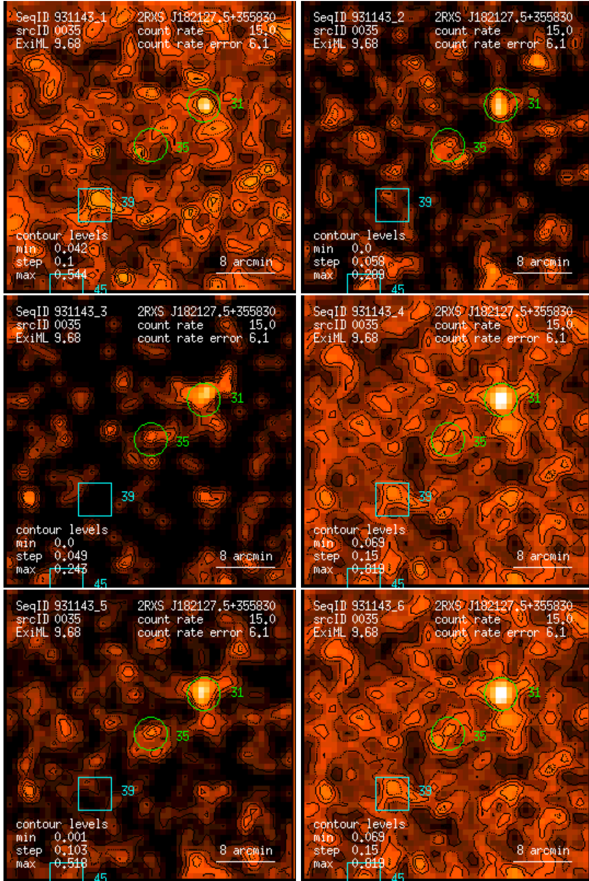
Figure 35: RASS 931143: detection 0035: band rate images, Gaussian filter: (1) PSPC channels 11 – 41, (2) 52 – 90, (3) 91 – 201, (4) 11 – 235, (5) 52 – 201, (6) 11 – 201. Broad band rates in counts/ks. Band rate contour levels in counts/ks/arcmin 2 .
