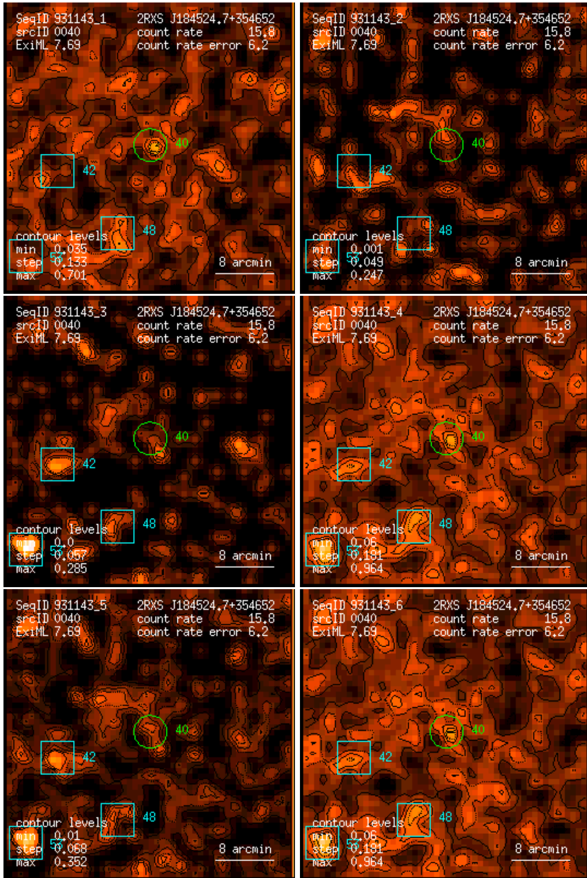
Figure 40: RASS 931143: detection 0040: band rate images, Gaussian filter: (1) PSPC channels 11 – 41, (2) 52 – 90, (3) 91 – 201, (4) 11 – 235, (5) 52 – 201, (6) 11 – 201. Broad band rates in counts/ks. Band rate contour levels in counts/ks/arcmin 2 .
