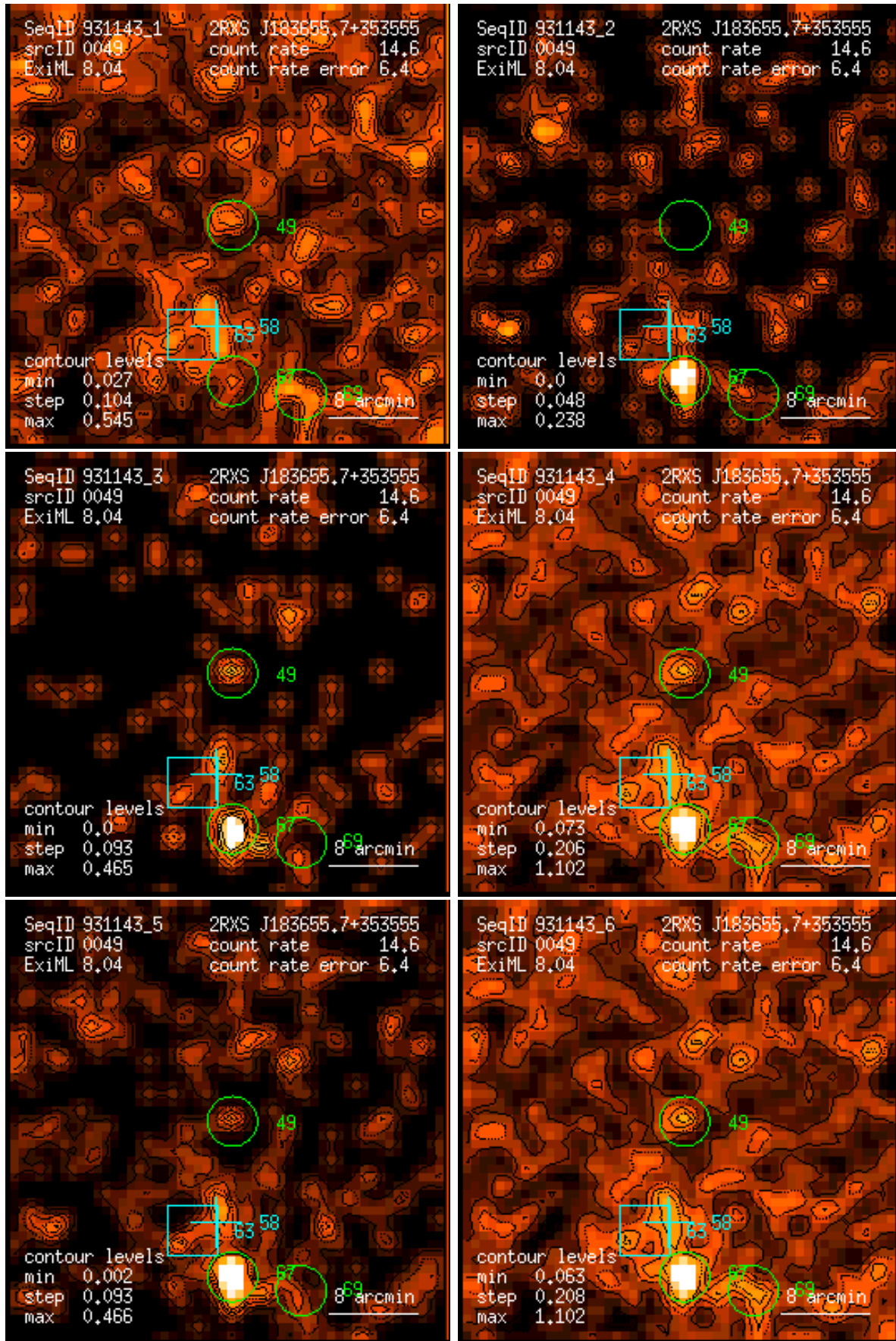
Figure 49: RASS 931143: detection 0049: band rate images, Gaussian filter: (1) PSPC channels 11 – 41, (2) 52 – 90, (3) 91 – 201, (4) 11 – 235, (5) 52 – 201, (6) 11 – 201. Broad band rates in counts/ks. Band rate contour levels in counts/ks/arcmin 2 .
