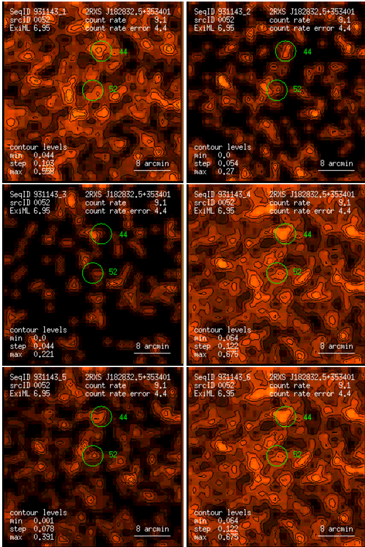
Figure 52: RASS 931143: detection 0052: band rate images, Gaussian filter: (1) PSPC channels 11 – 41, (2) 52 – 90, (3) 91 – 201, (4) 11 – 235, (5) 52 – 201, (6) 11 – 201. Broad band rates in counts/ks. Band rate contour levels in counts/ks/arcmin 2 .
