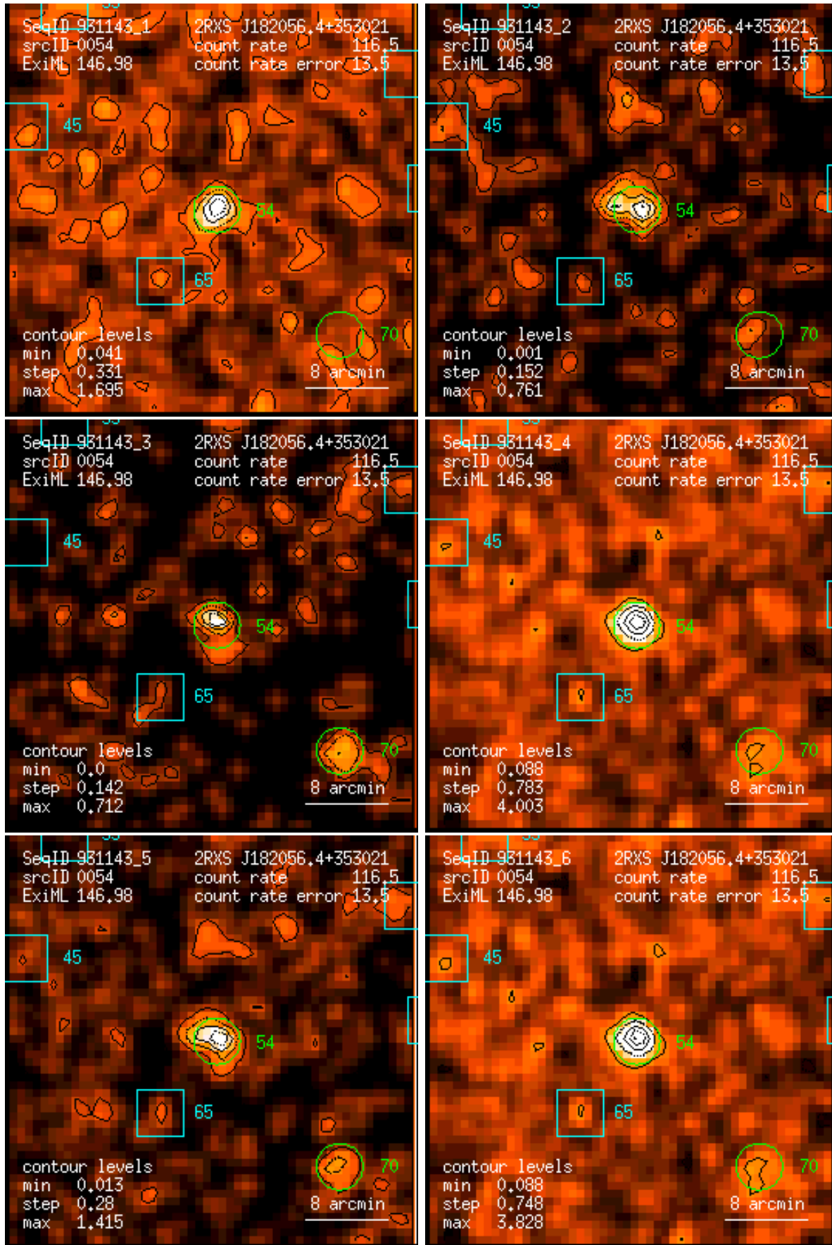
Figure 54: RASS 931143: detection 0054: band rate images, Gaussian filter: (1) PSPC channels 11 – 41, (2) 52 – 90, (3) 91 – 201, (4) 11 – 235, (5) 52 – 201, (6) 11 – 201. Broad band rates in counts/ks. Band rate contour levels in counts/ks/arcmin 2 .
